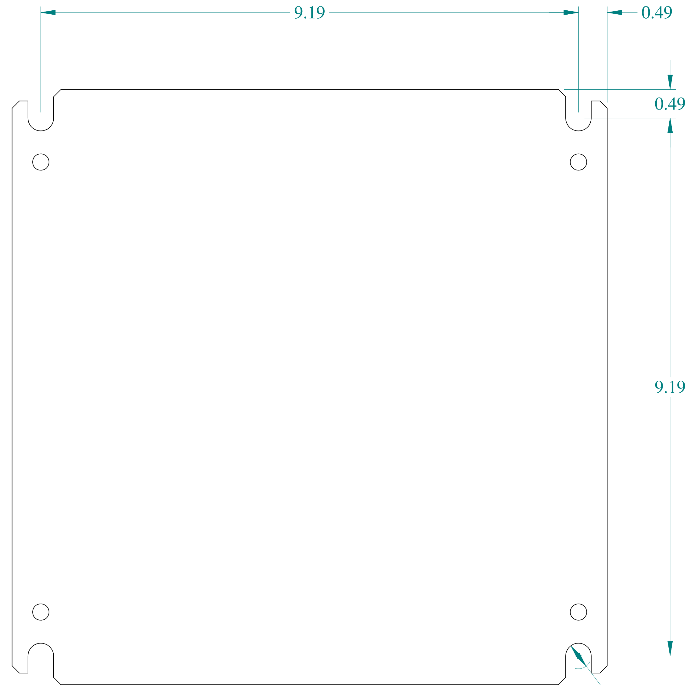
FRONT VIEW
