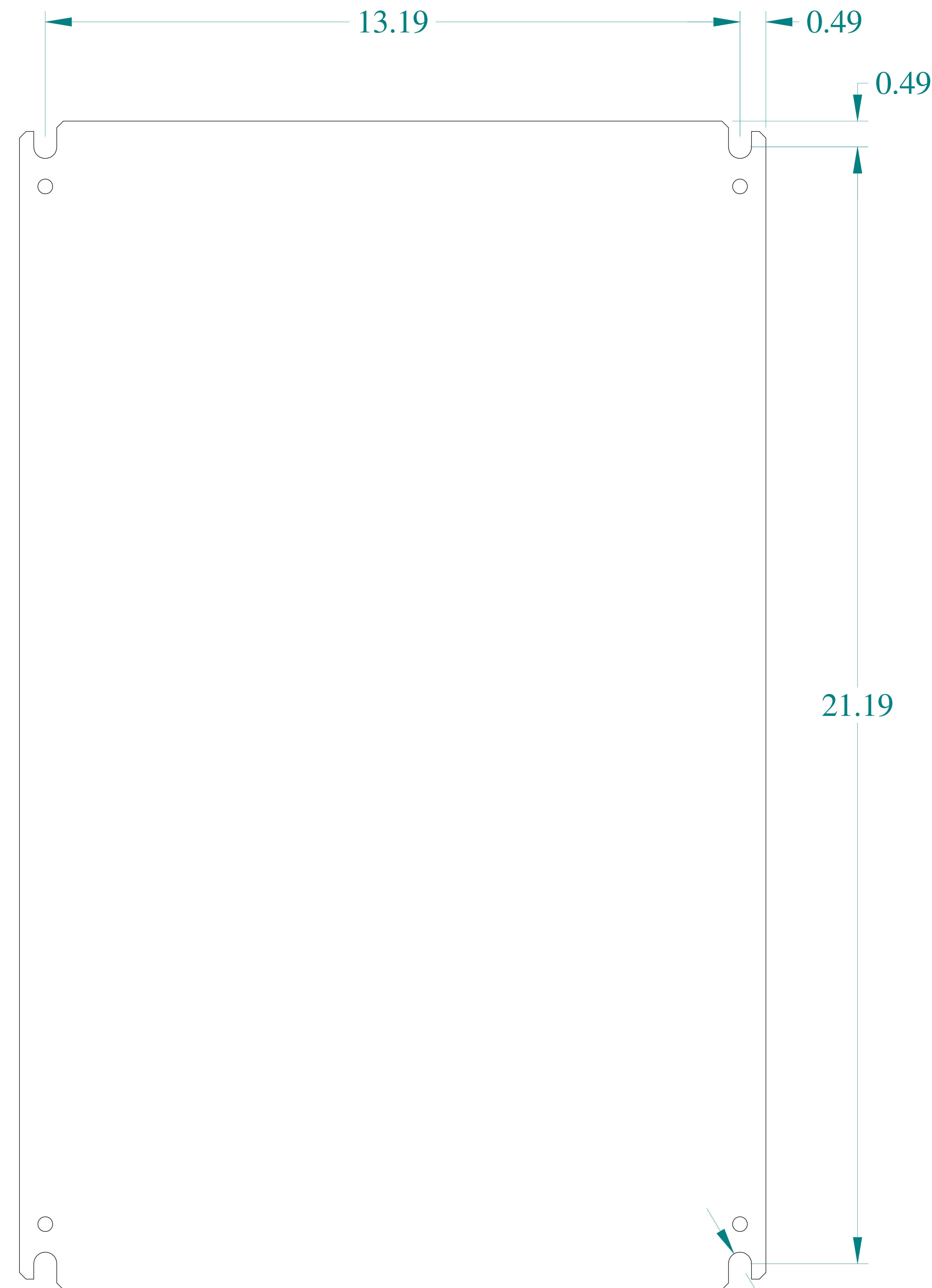
FRONT VIEW
