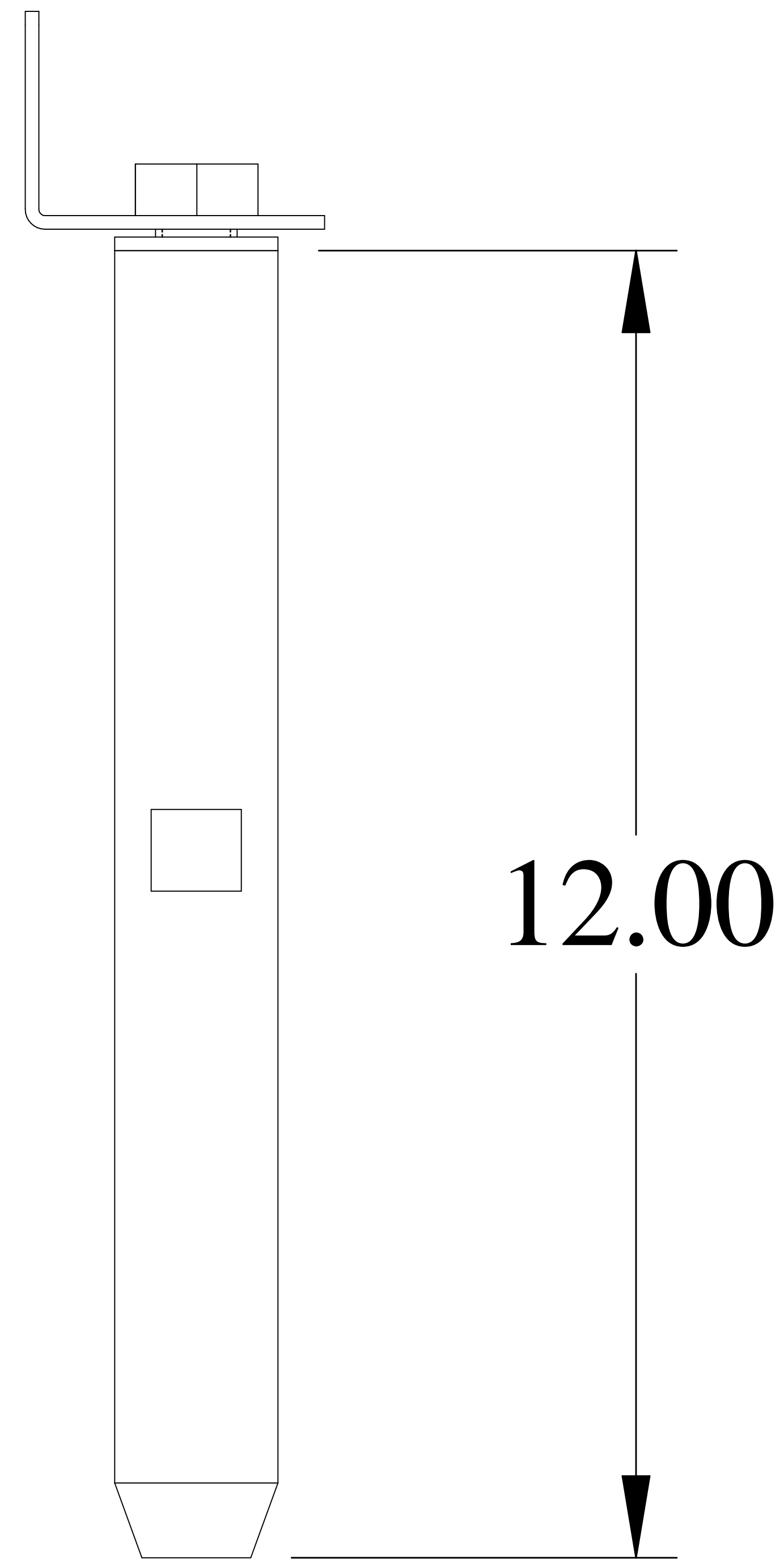
FRONT VIEW
