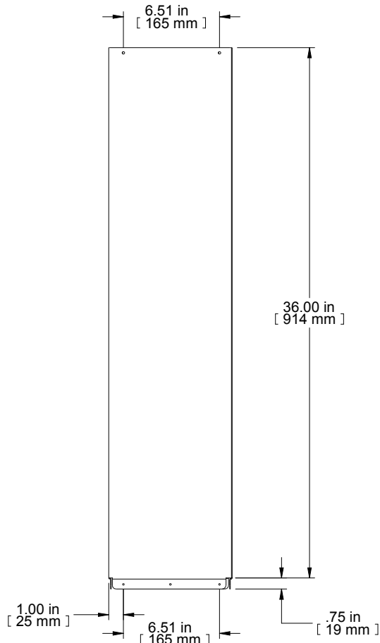
R.S. VIEW
