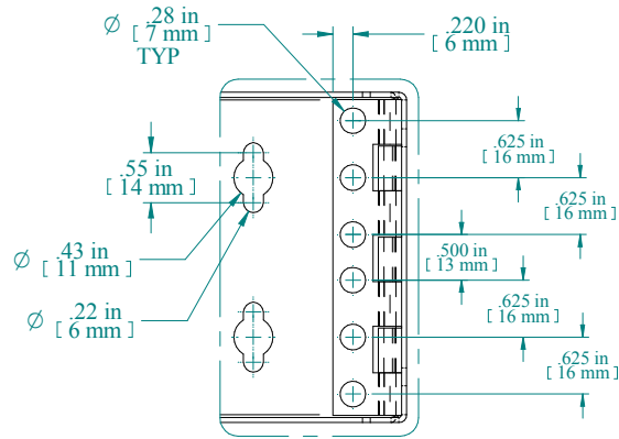
DETAIL A 3:1
