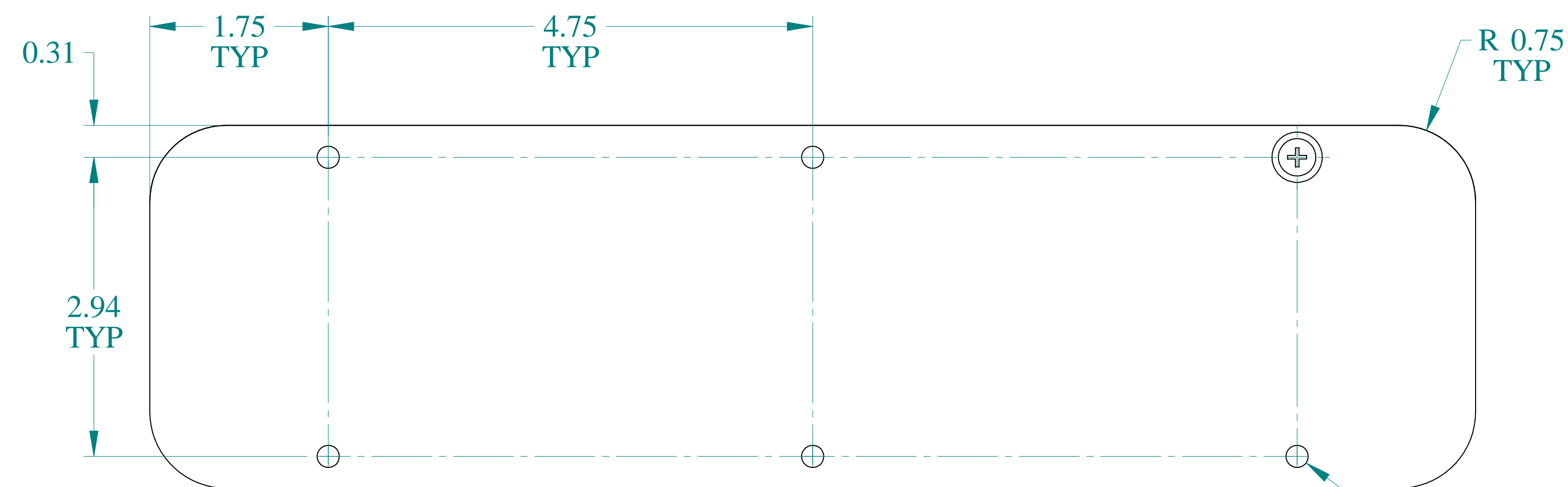
FRONT VIEW
