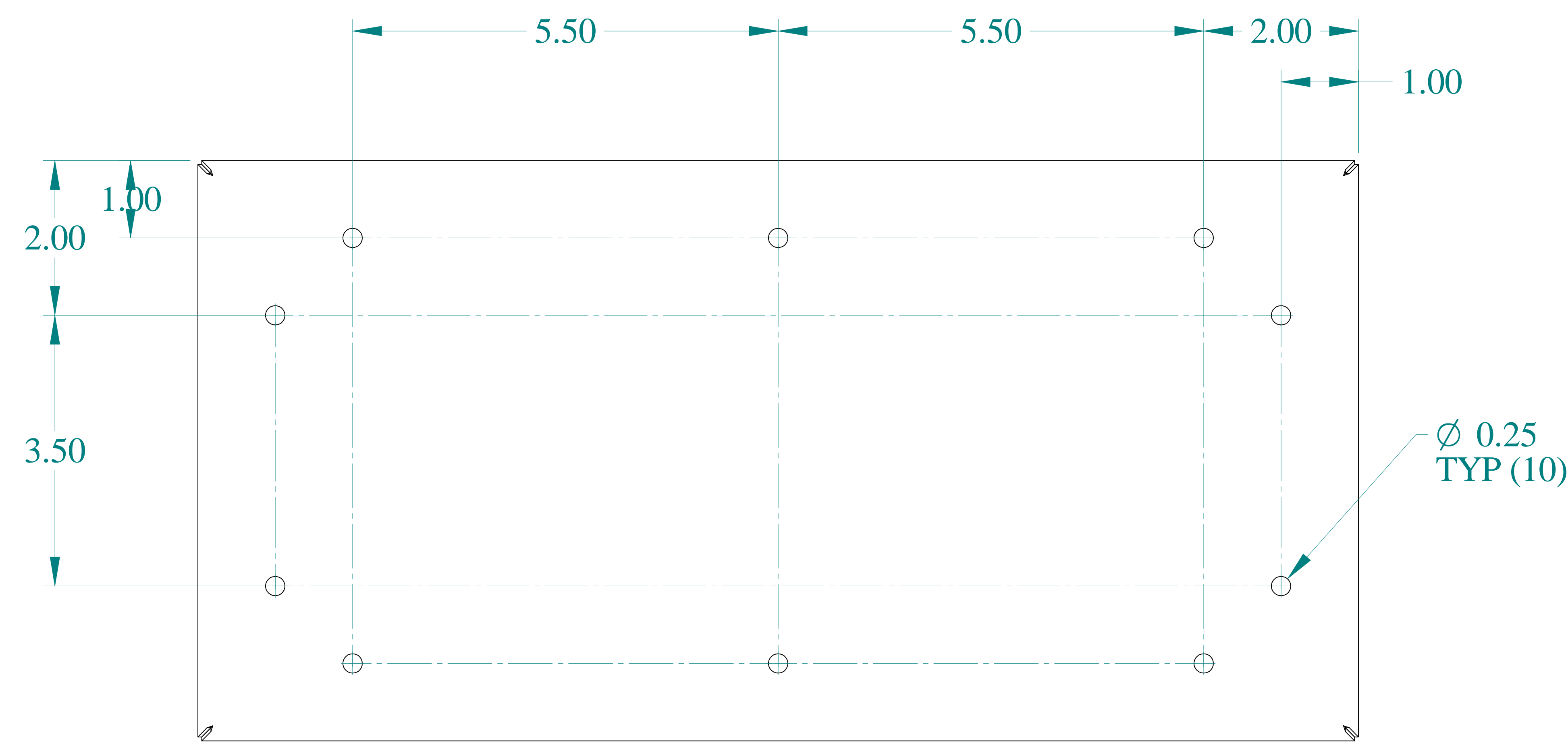
FRONT VIEW
