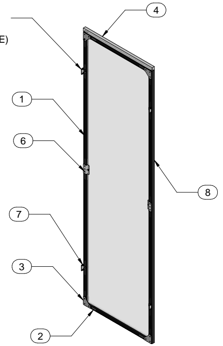
ISOMETRIC
