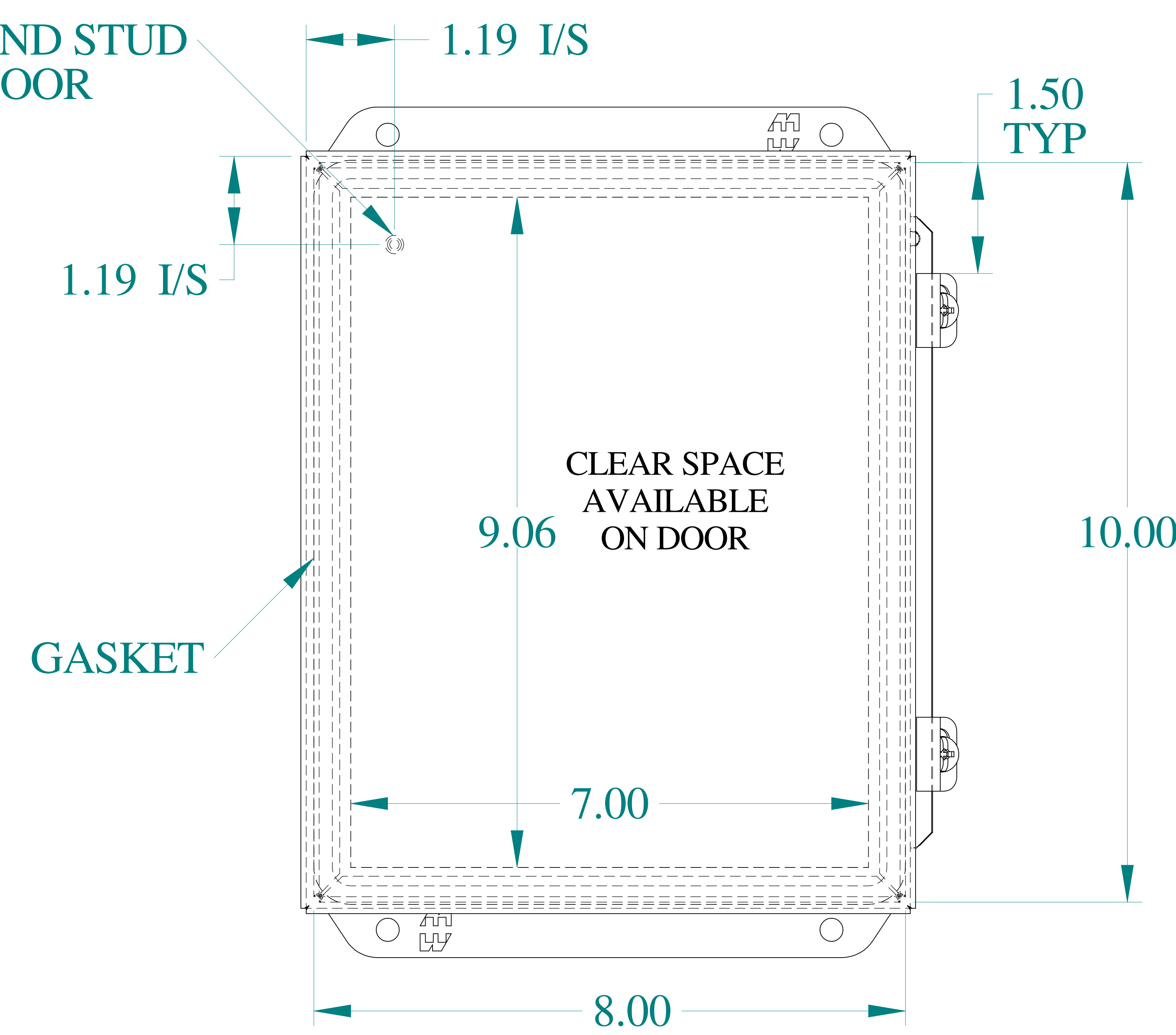
FRONT VIEW
