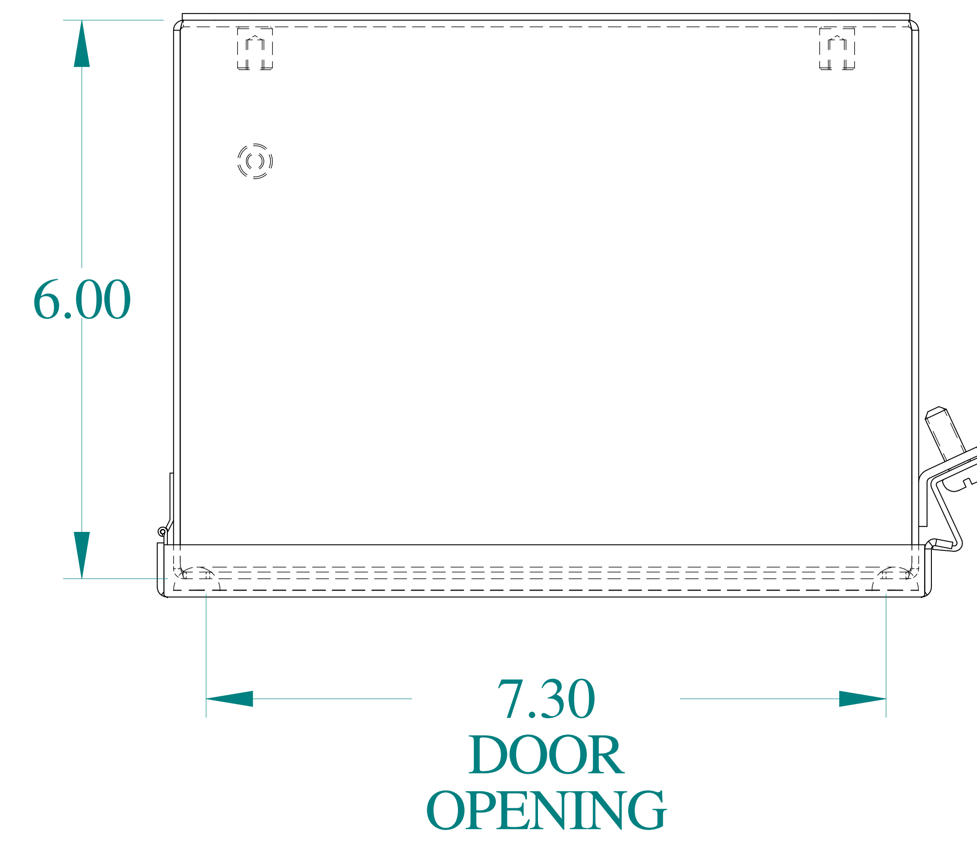
TOP VIEW
