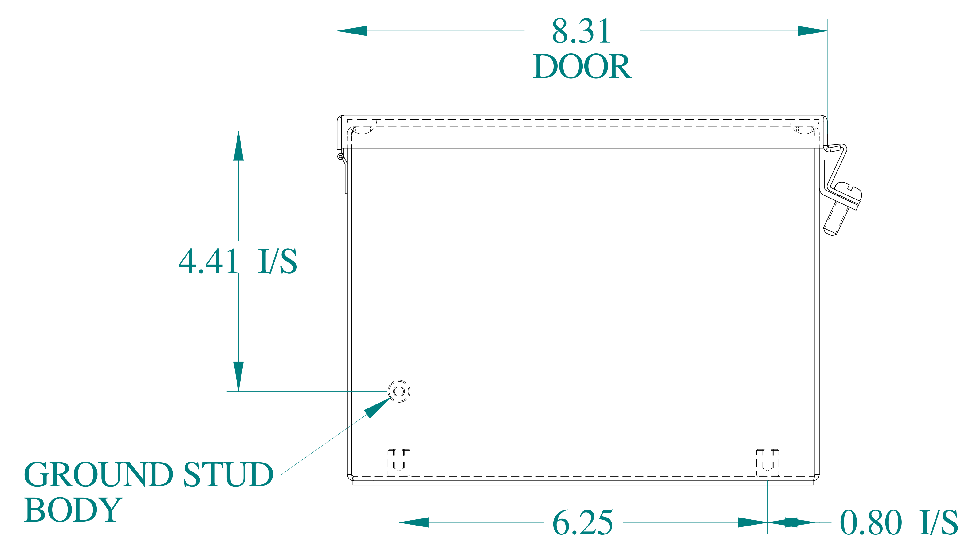
BOTTOM VIEW
