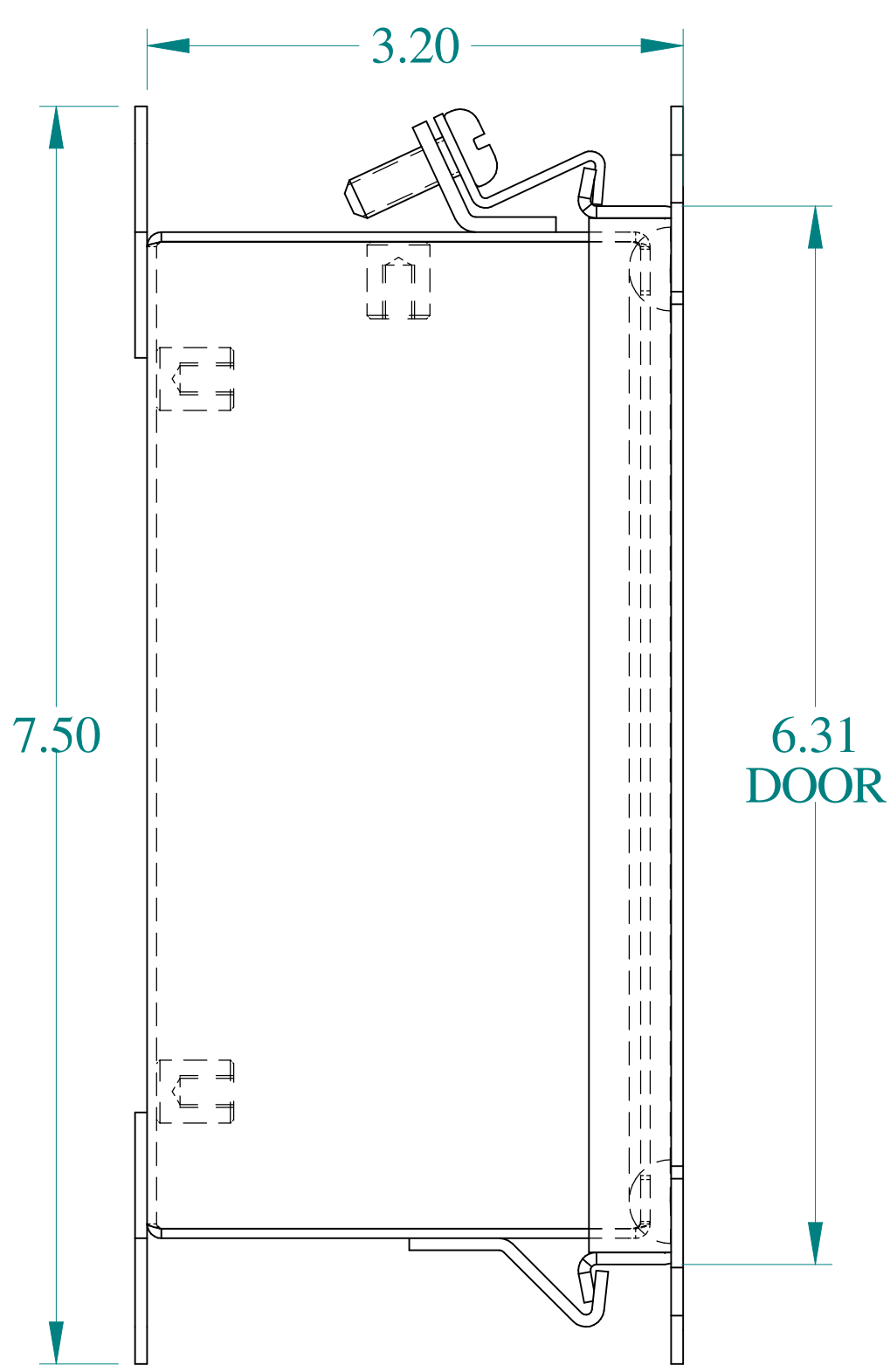
SIDE VIEW
