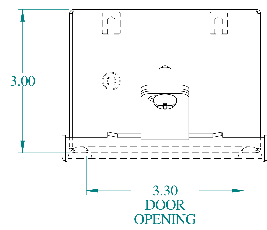
TOP VIEW
