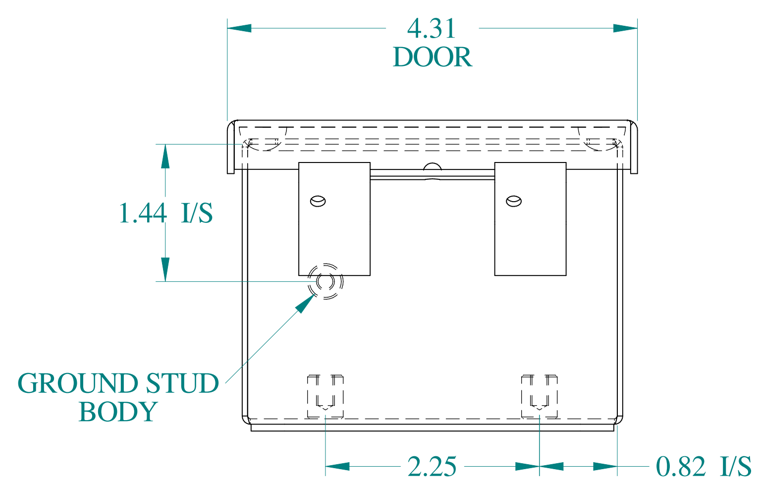
BOTTOM VIEW
