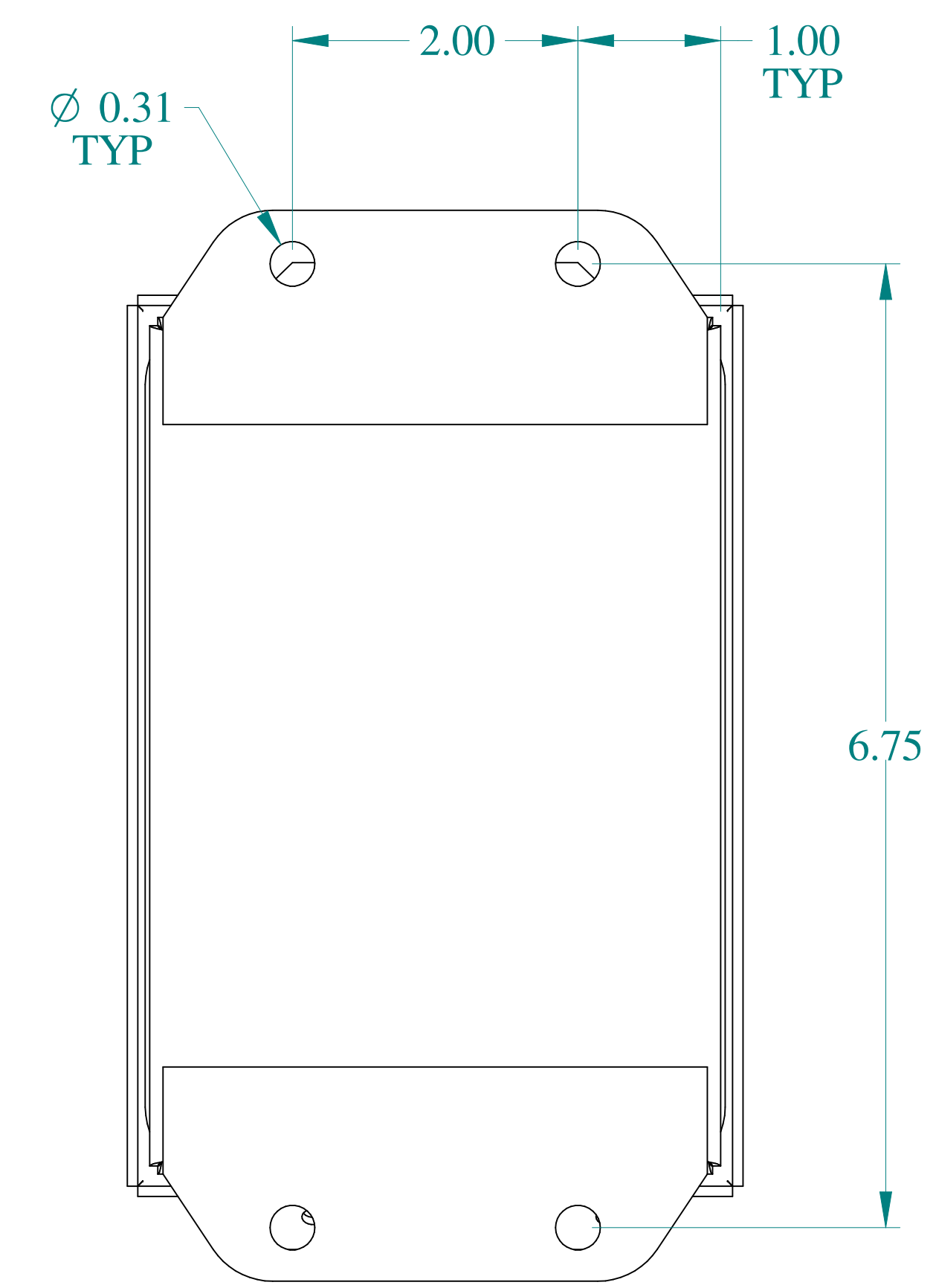
BACK VIEW
