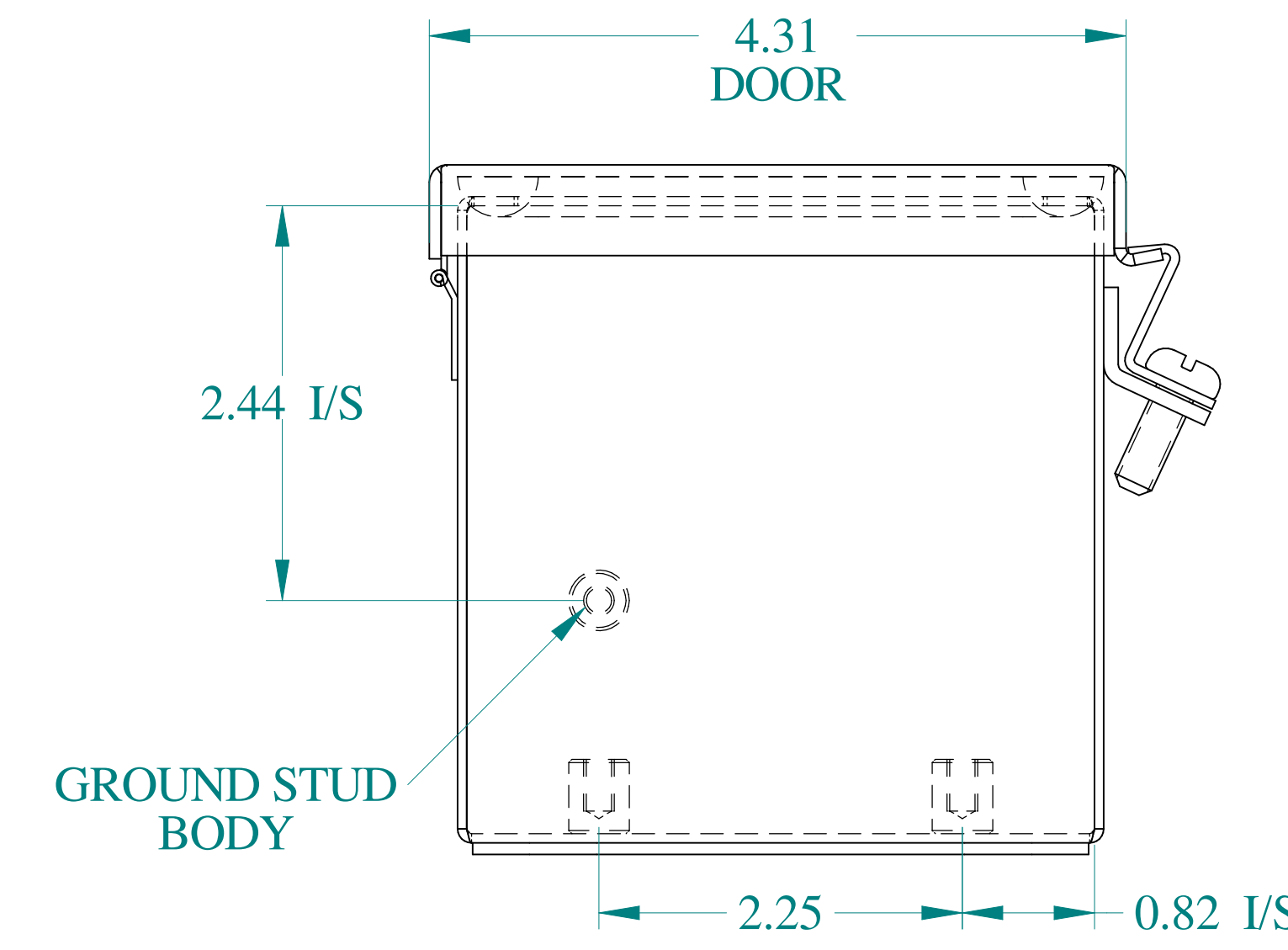
BOTTOM VIEW
