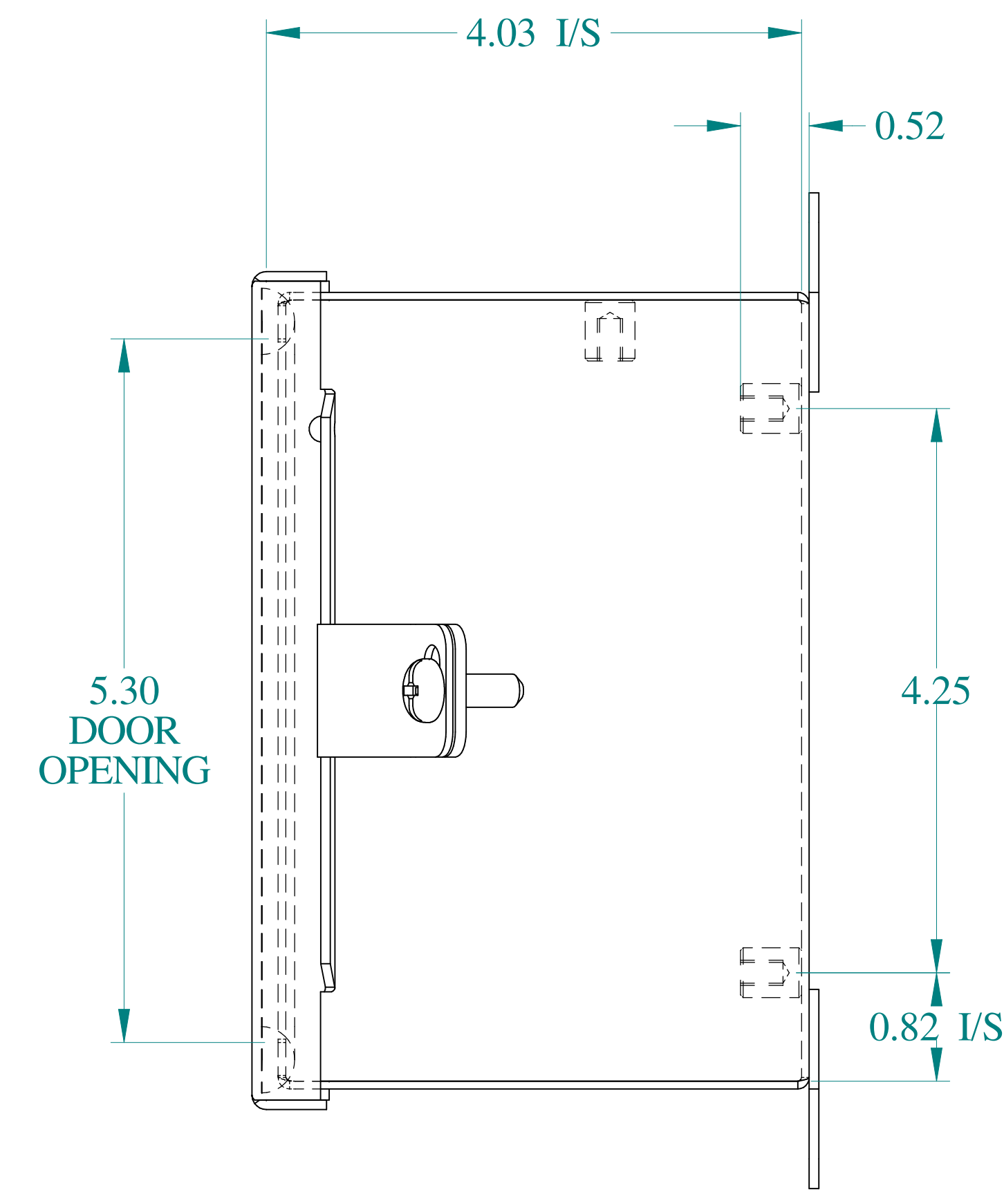
SIDE VIEW
