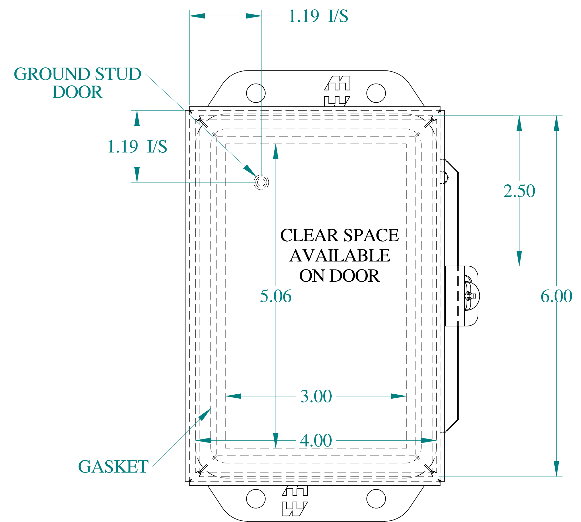
FRONT VIEW
