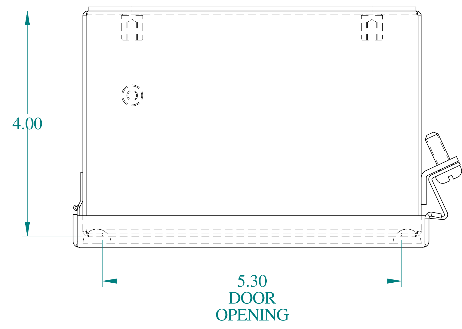
TOP VIEW
