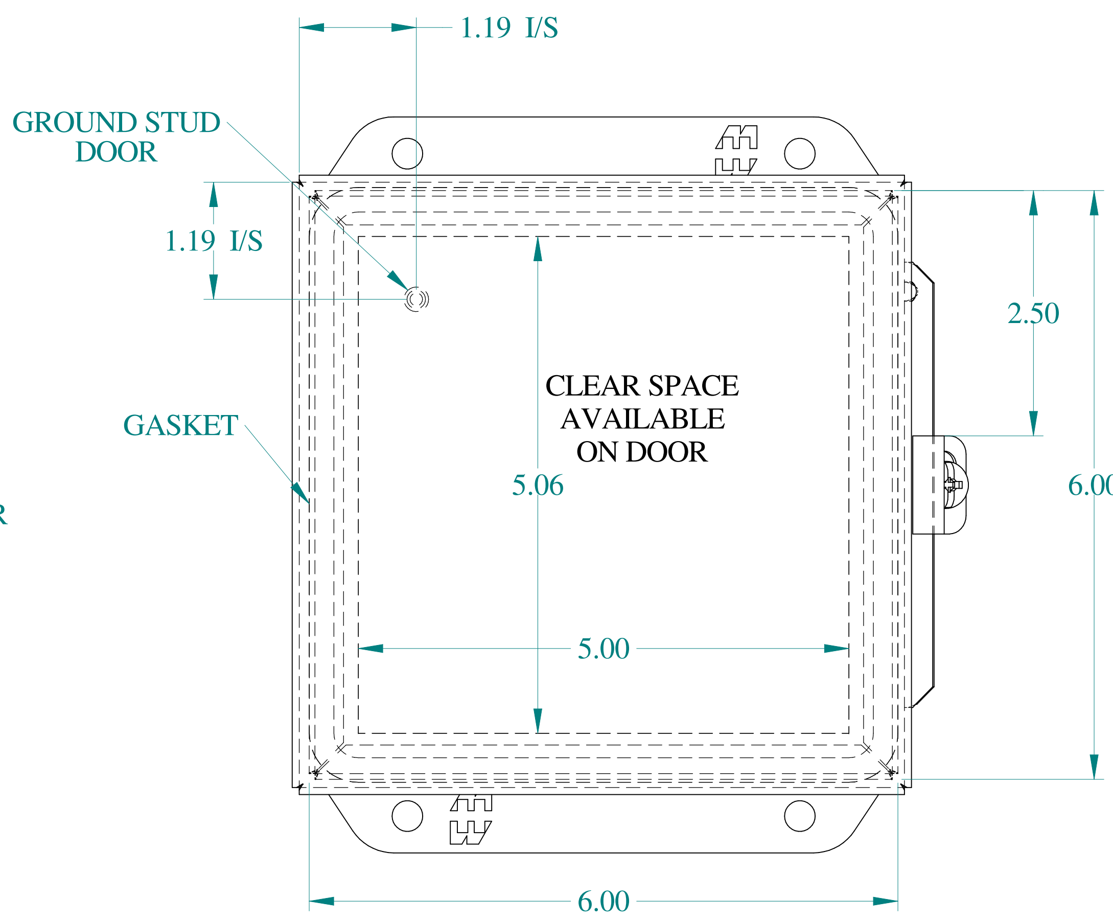
FRONT VIEW
