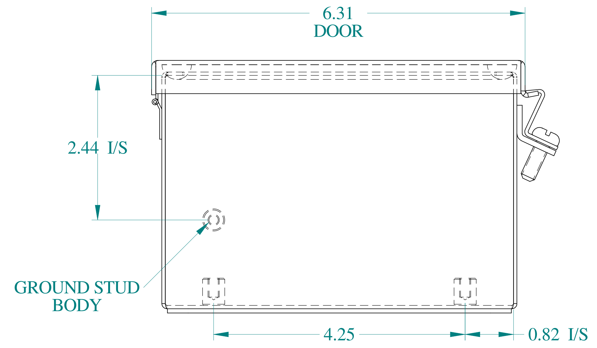
BOTTOM VIEW
