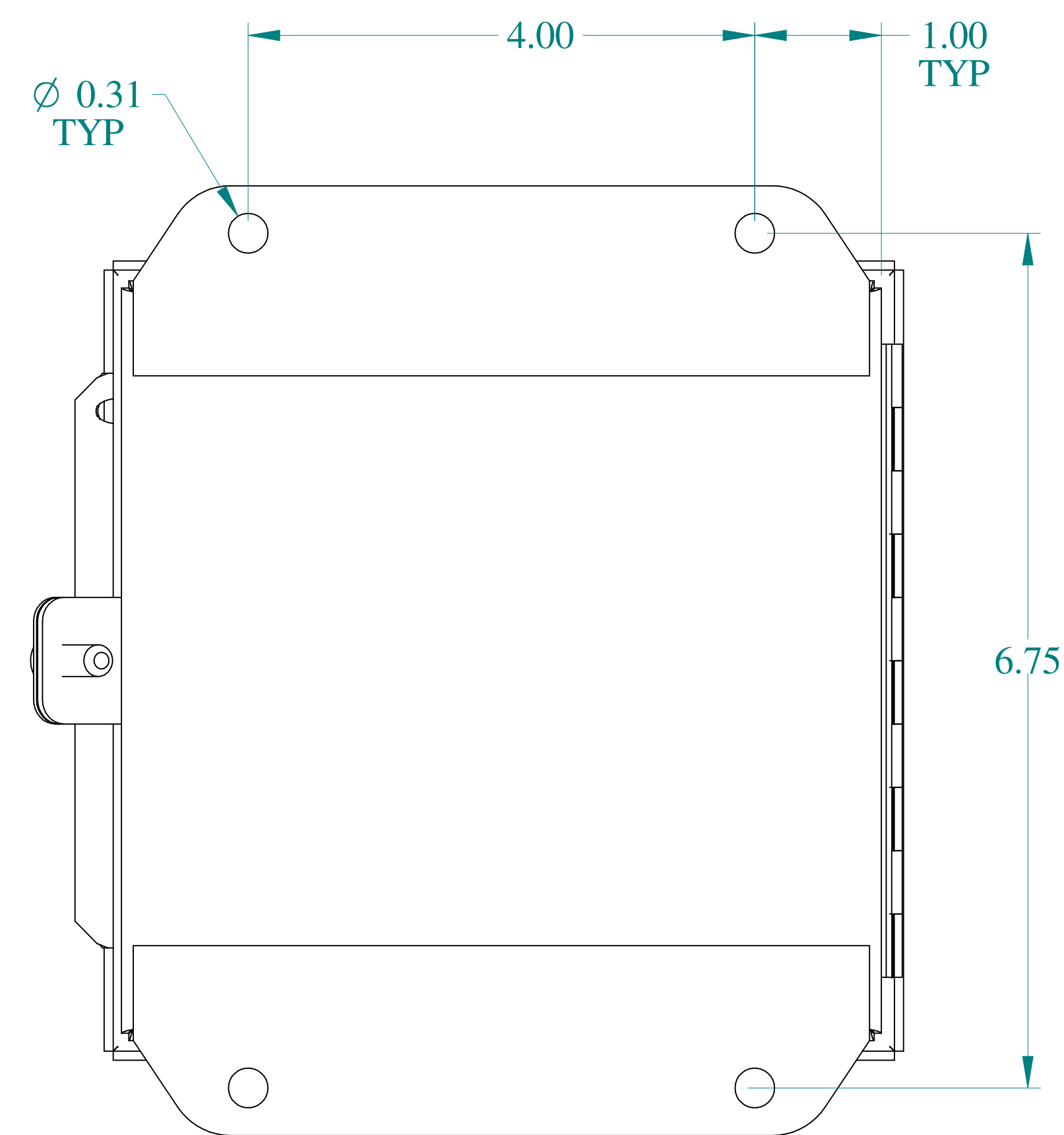
BACK VIEW
