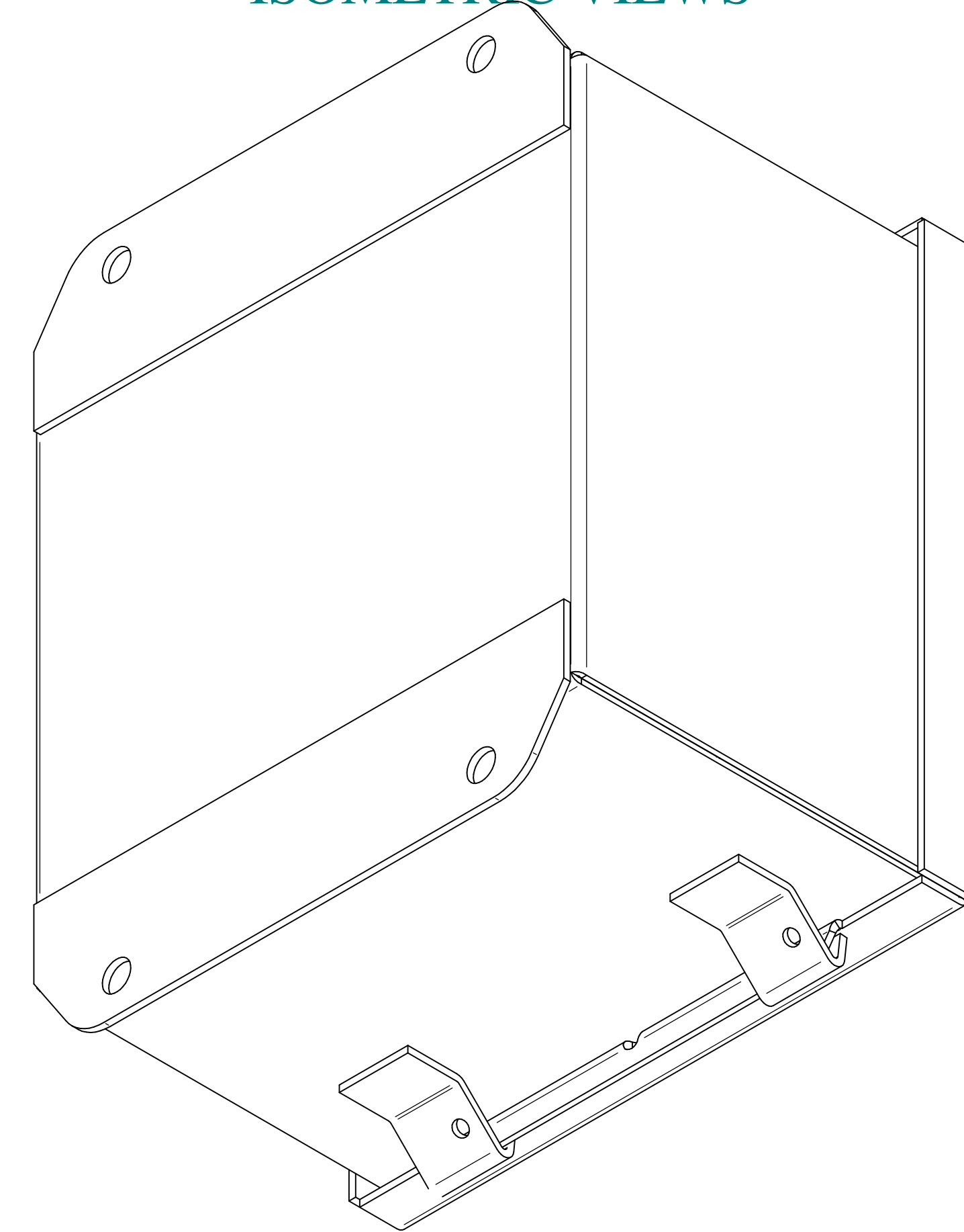
ISOMETRIC VIEWS
