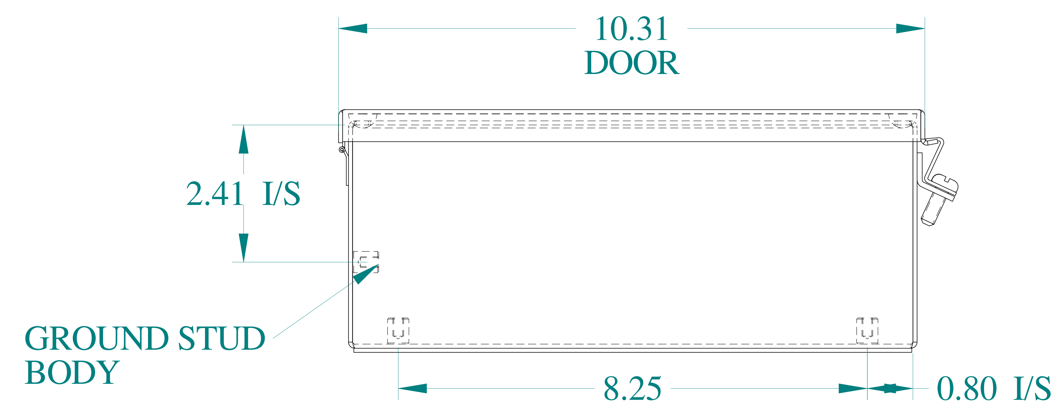
BOTTOM VIEW
