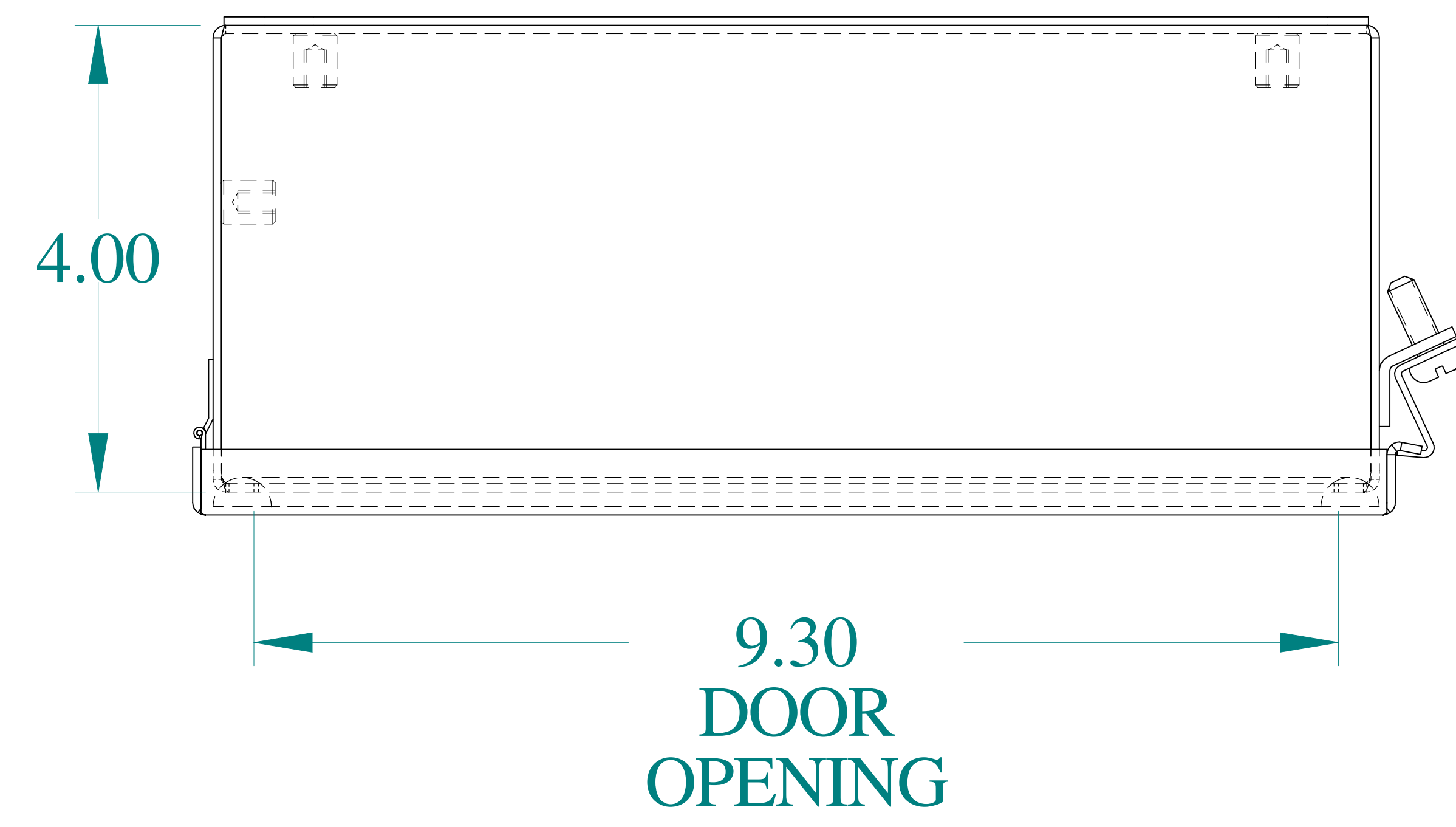
TOP VIEW
