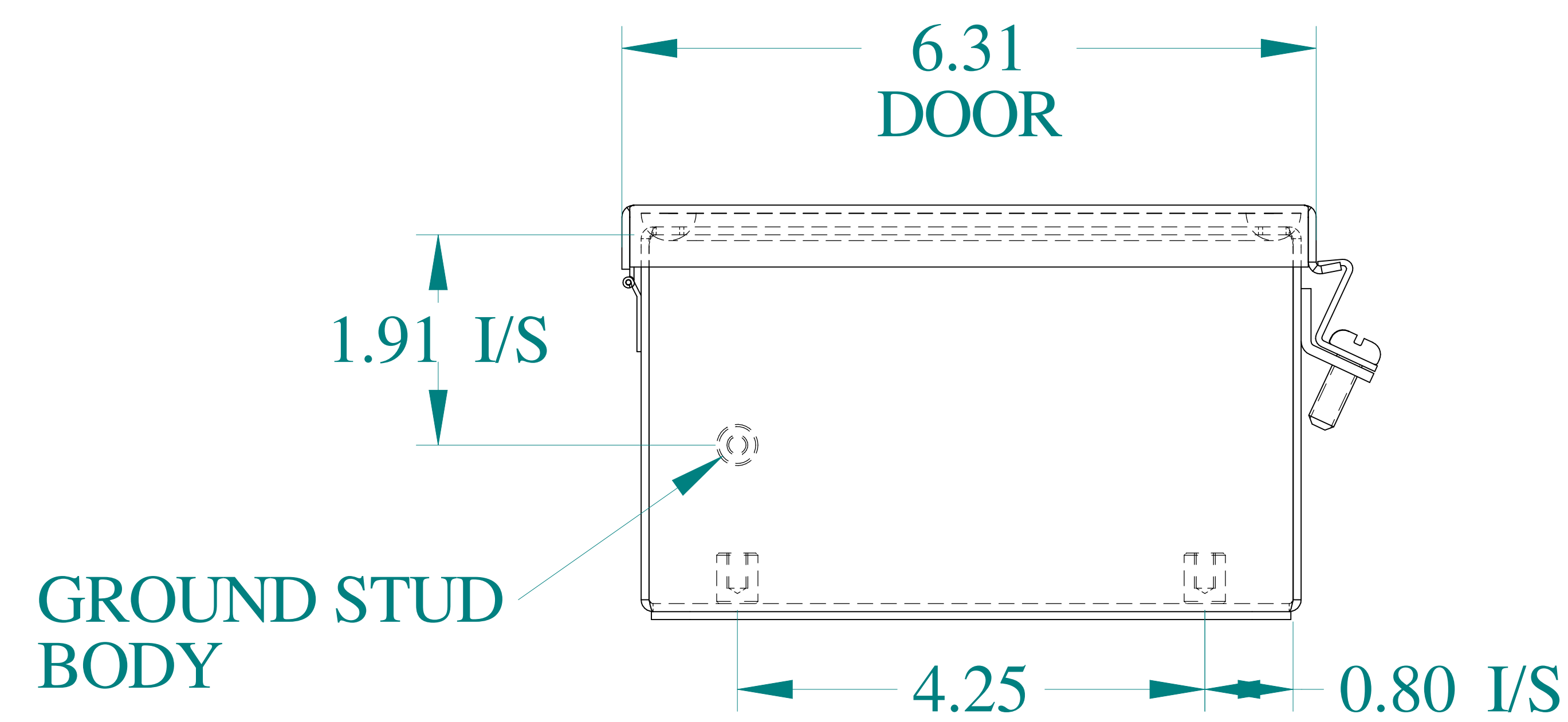
BOTTOM VIEW
