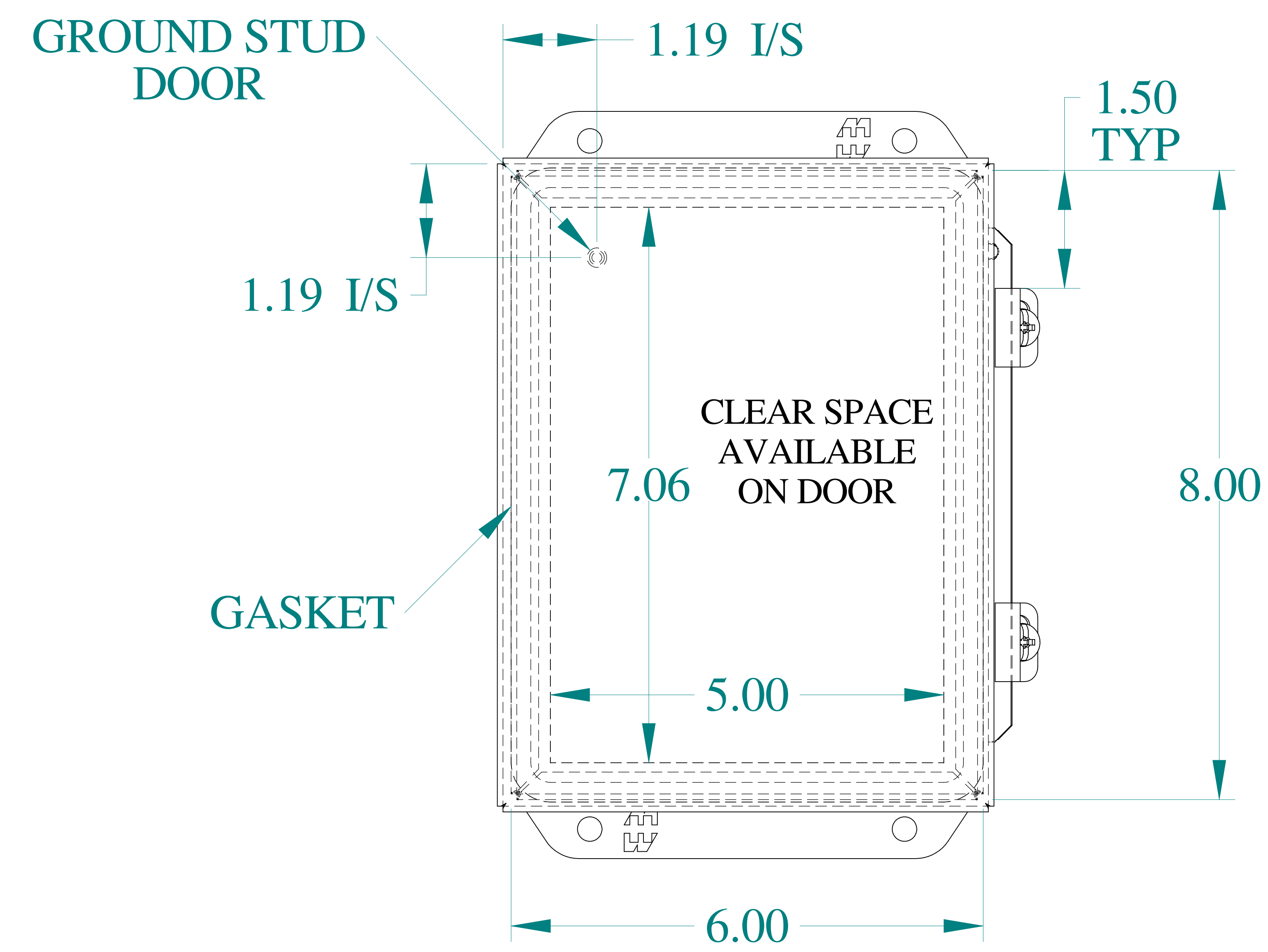
FRONT VIEW
