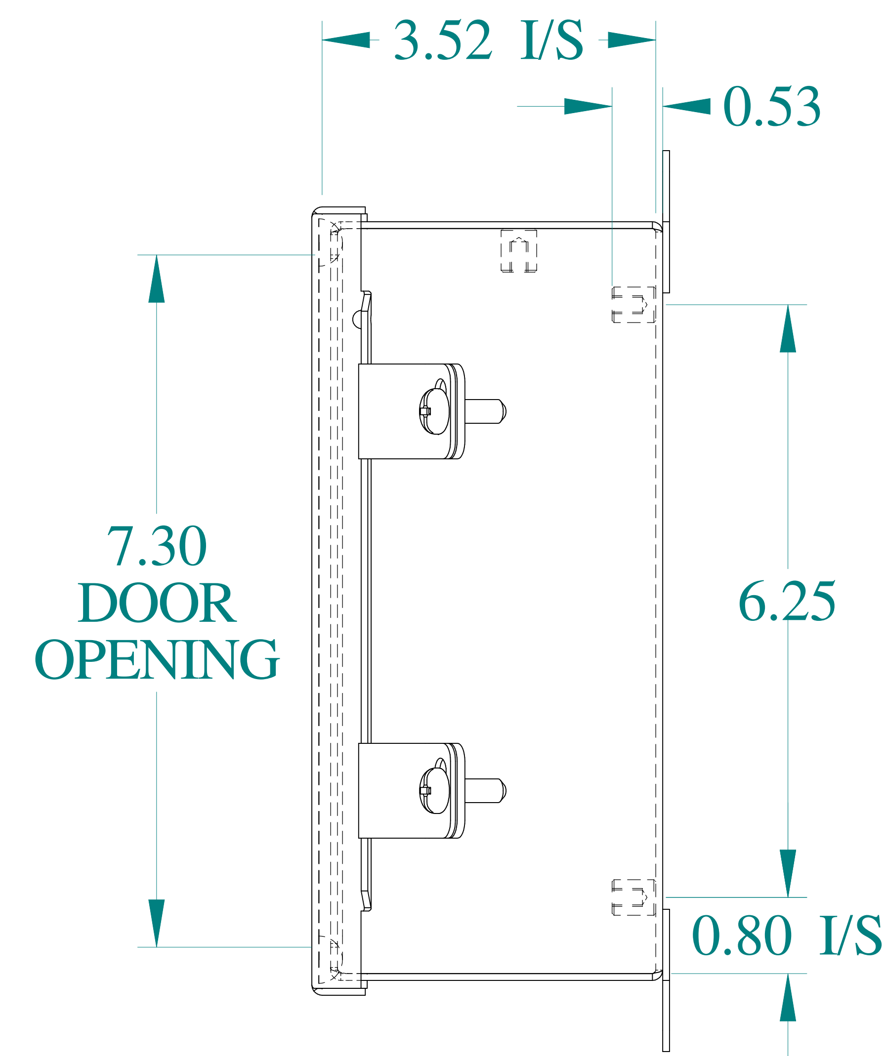
SIDE VIEW
