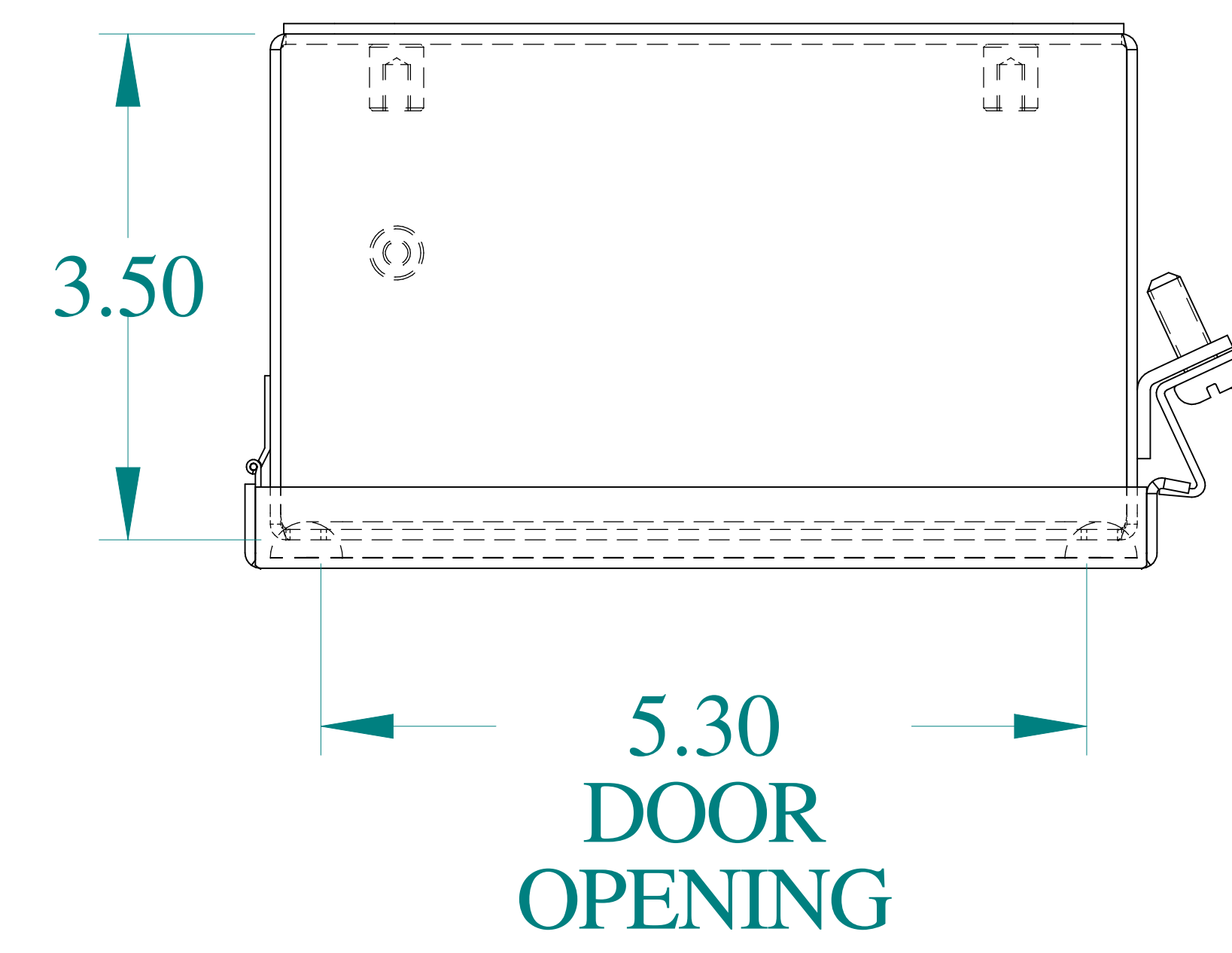
TOP VIEW
