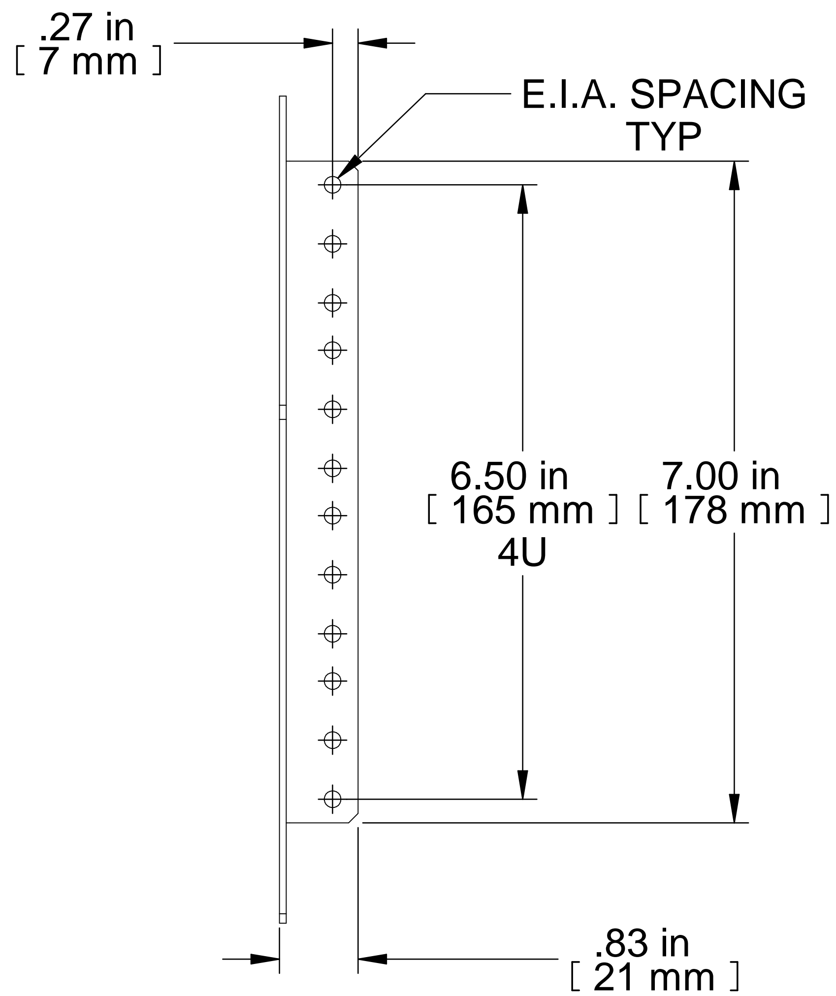
FRONT VIEW
