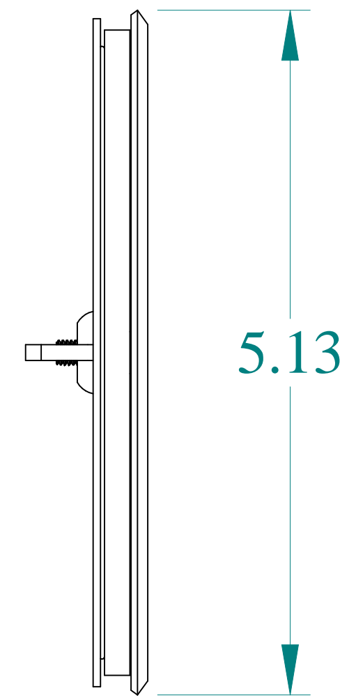
SIDE VIEW
