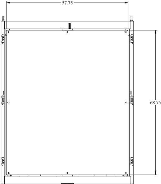
FRONT DOOR REMOVED
