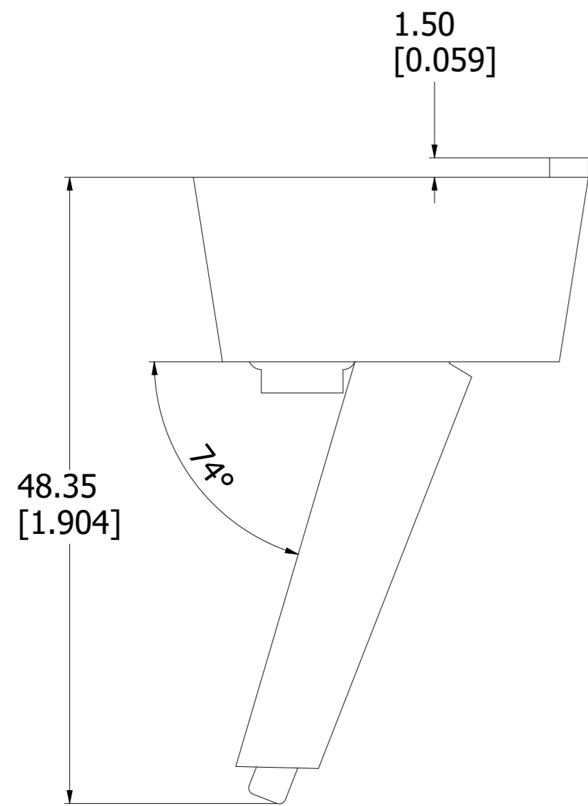
SIDE VIEW w/ LEG FOLDED DOWN
