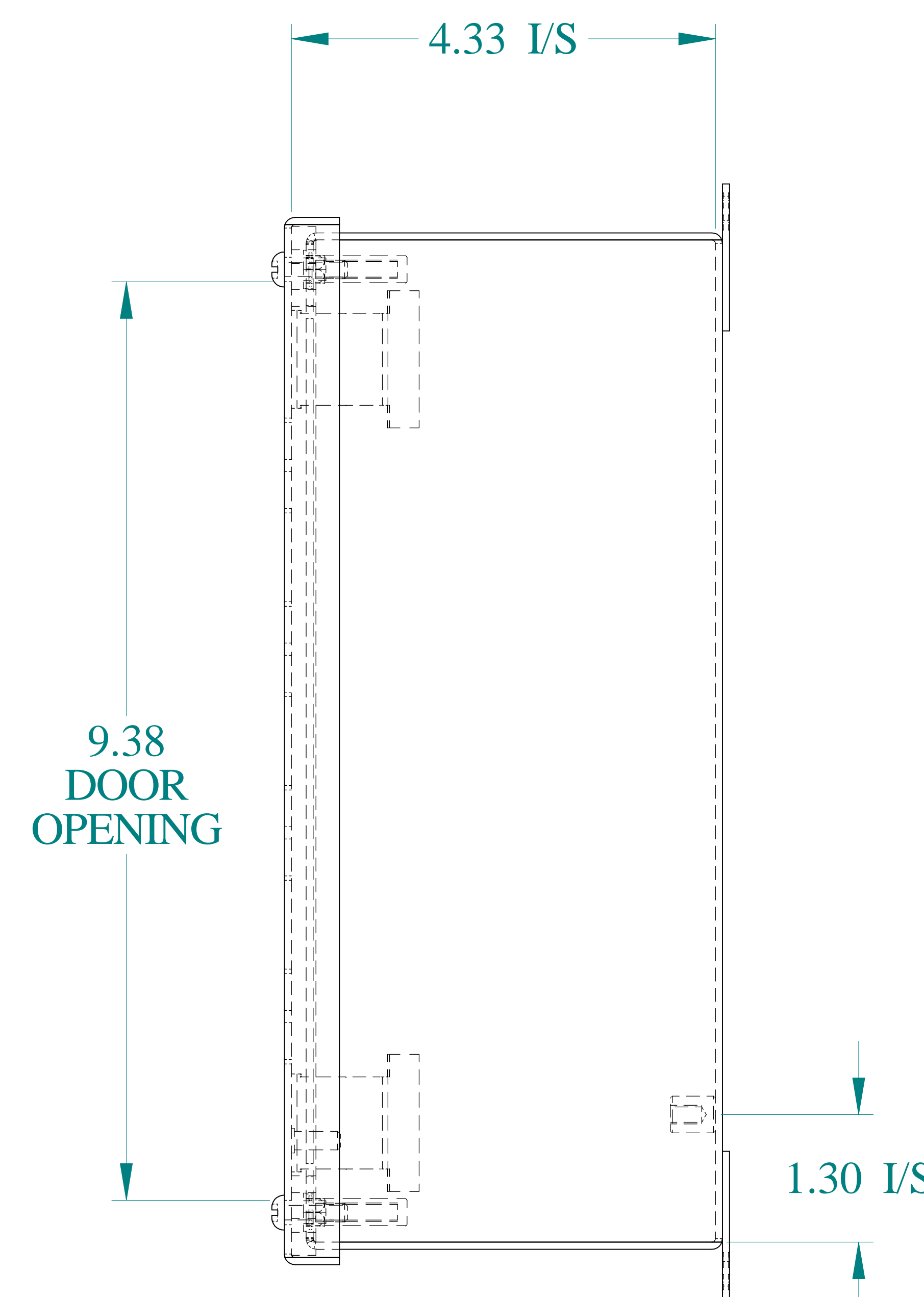
SIDE VIEW
