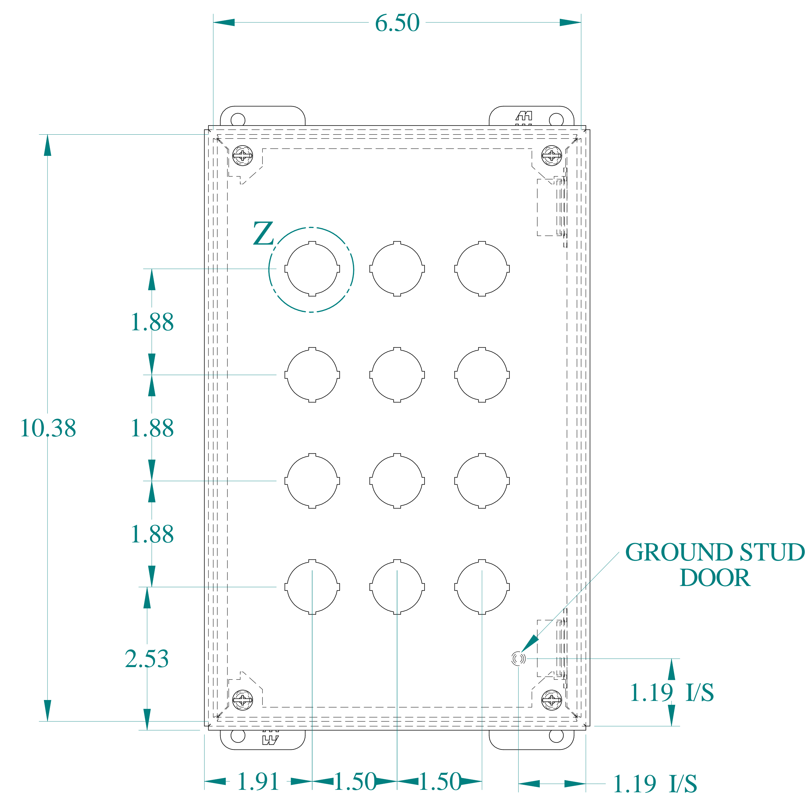
FRONT VIEW
