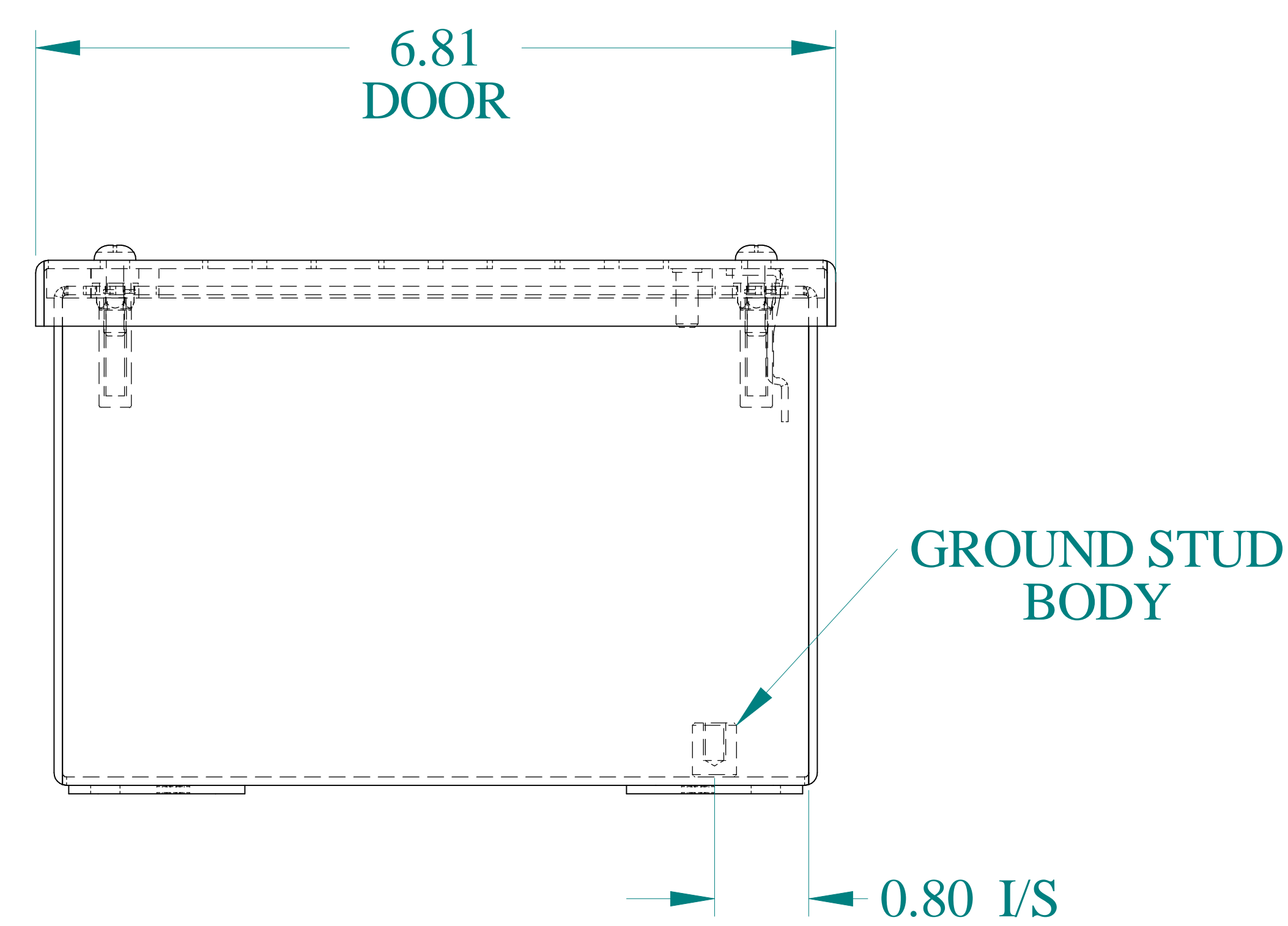
BOTTOM VIEW
