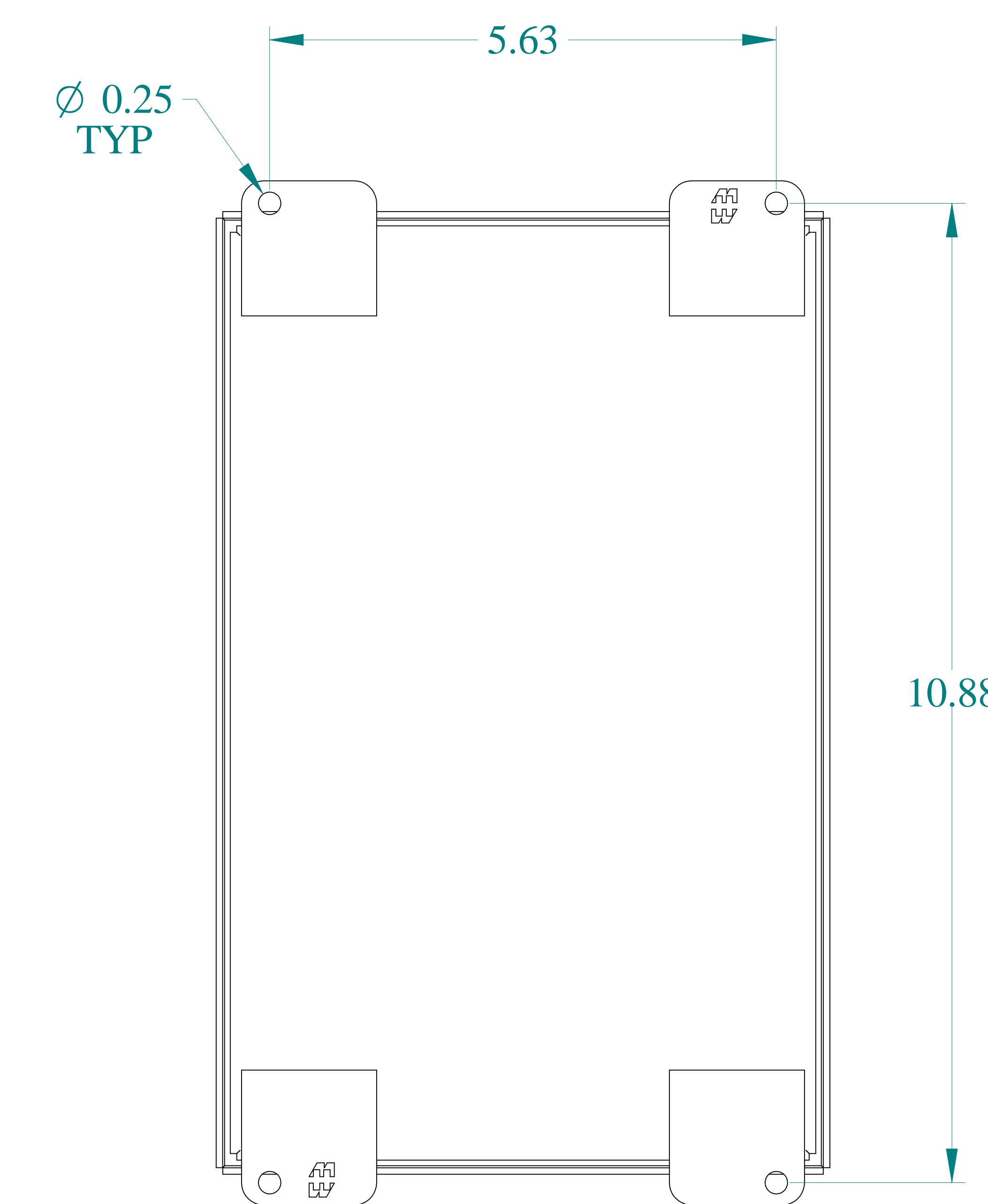
BACK VIEW
