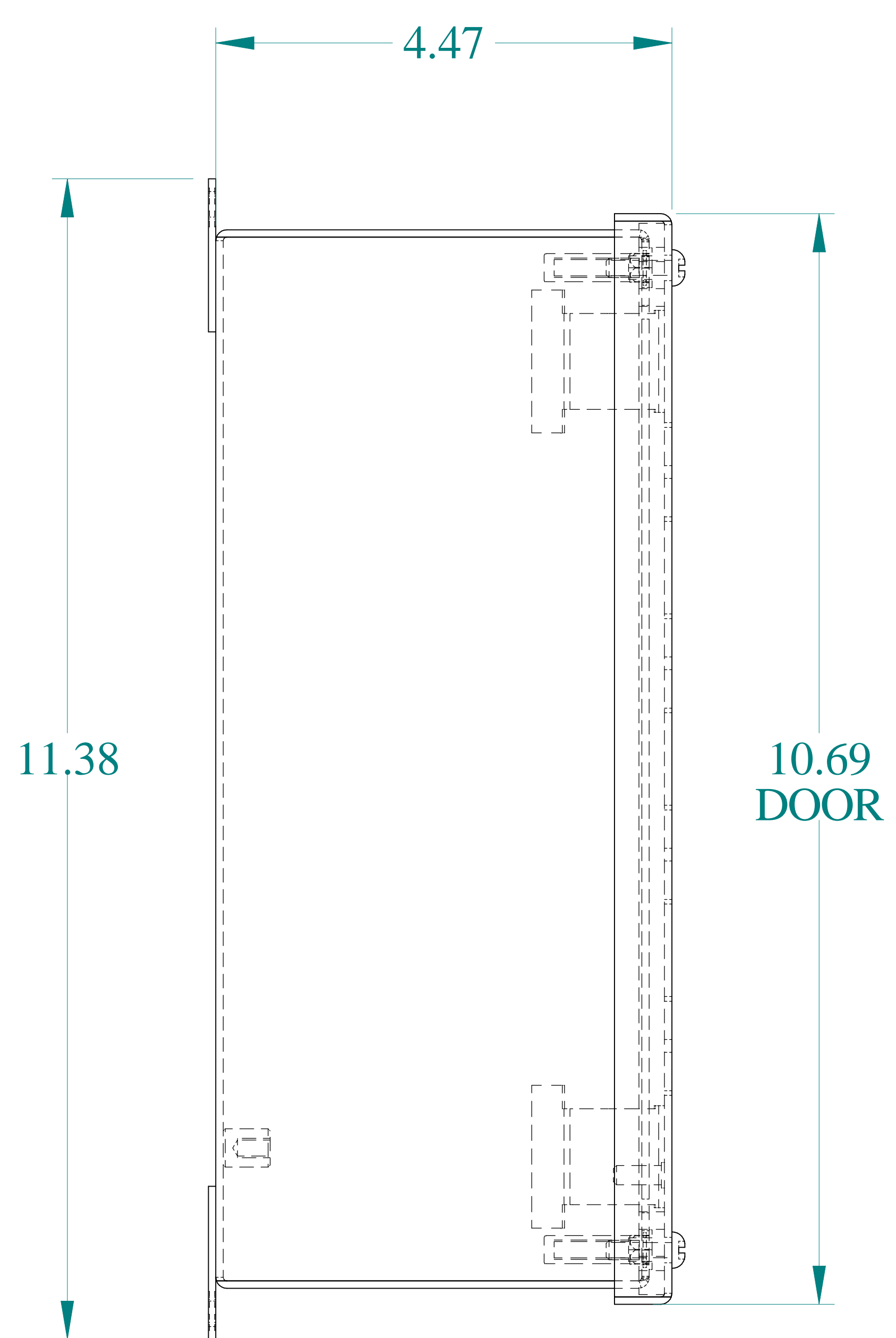
SIDE VIEW
