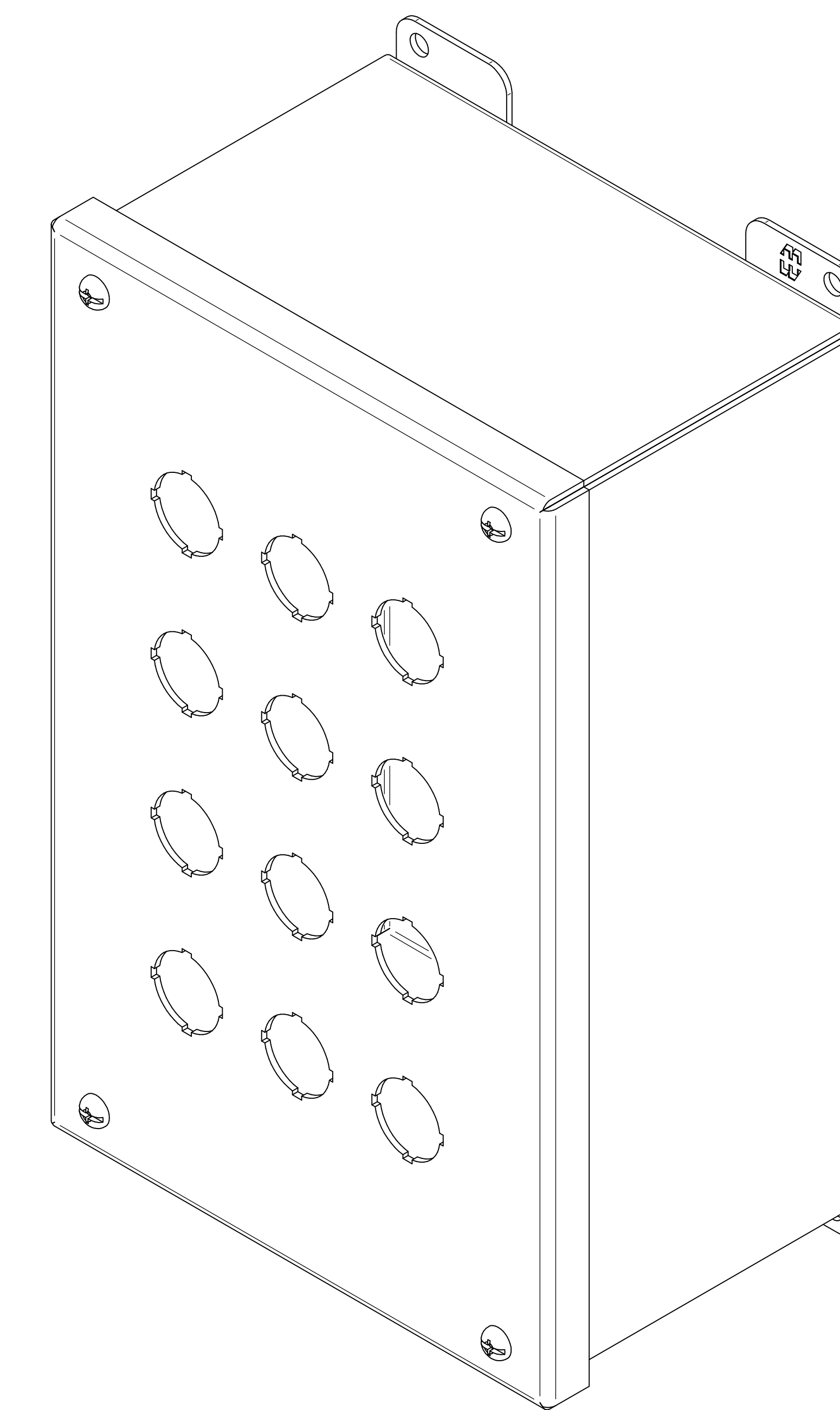
ISOMETRIC VIEWS
