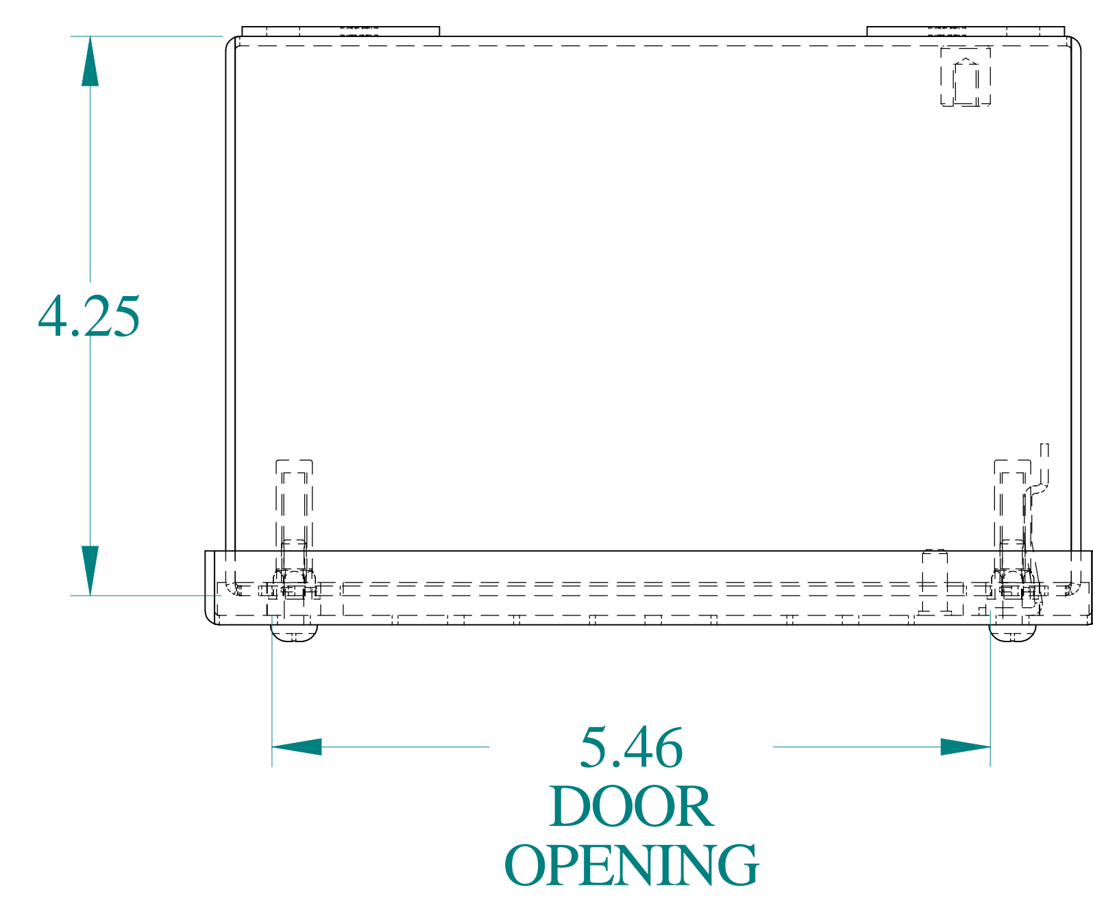
TOP VIEW
