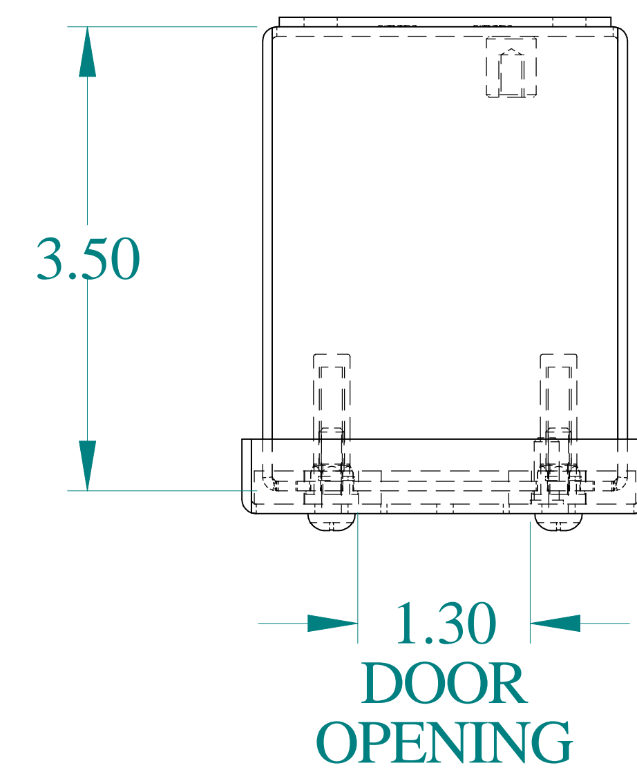
TOP VIEW
