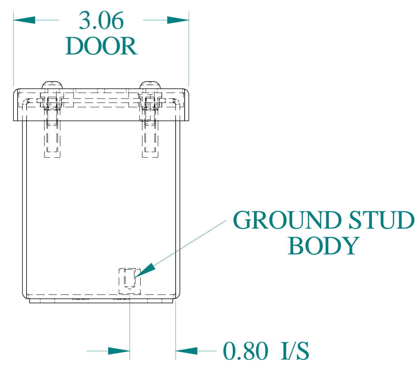
BOTTOM VIEW
