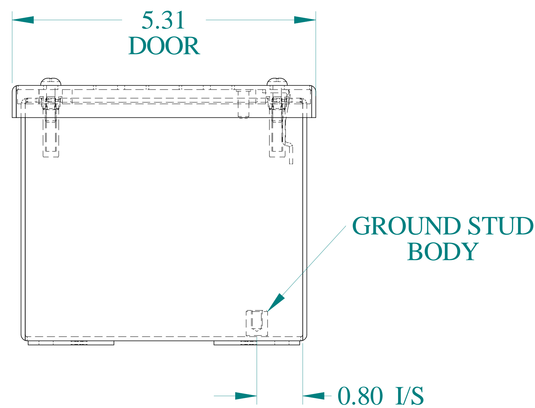
BOTTOM VIEW
