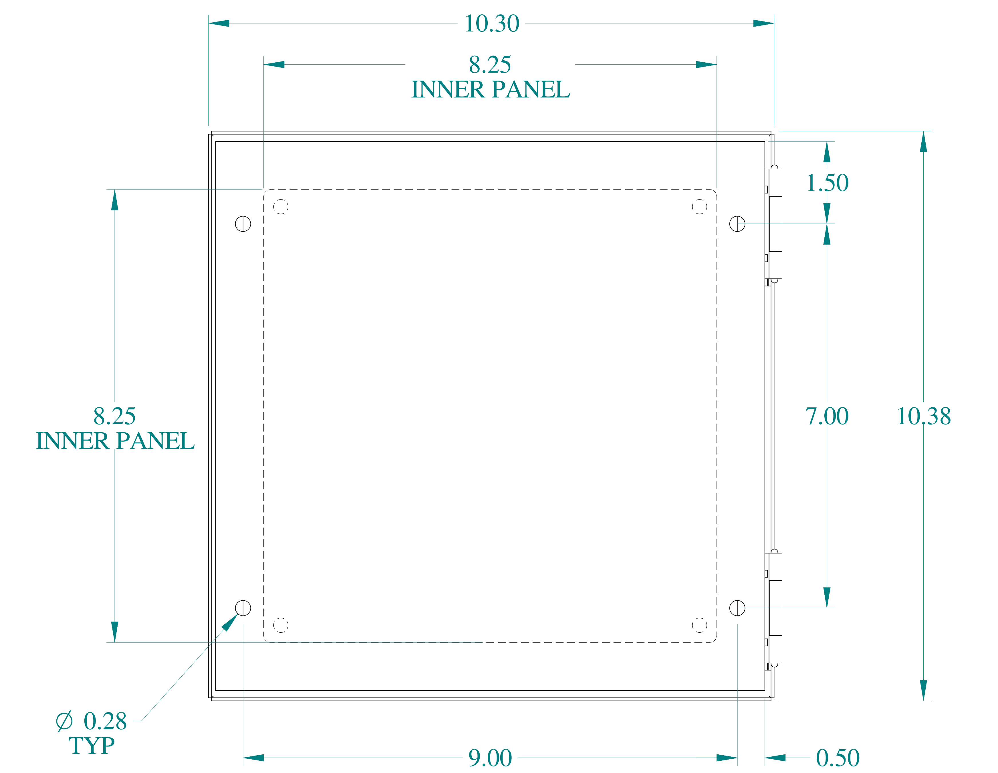
BACK VIEW
