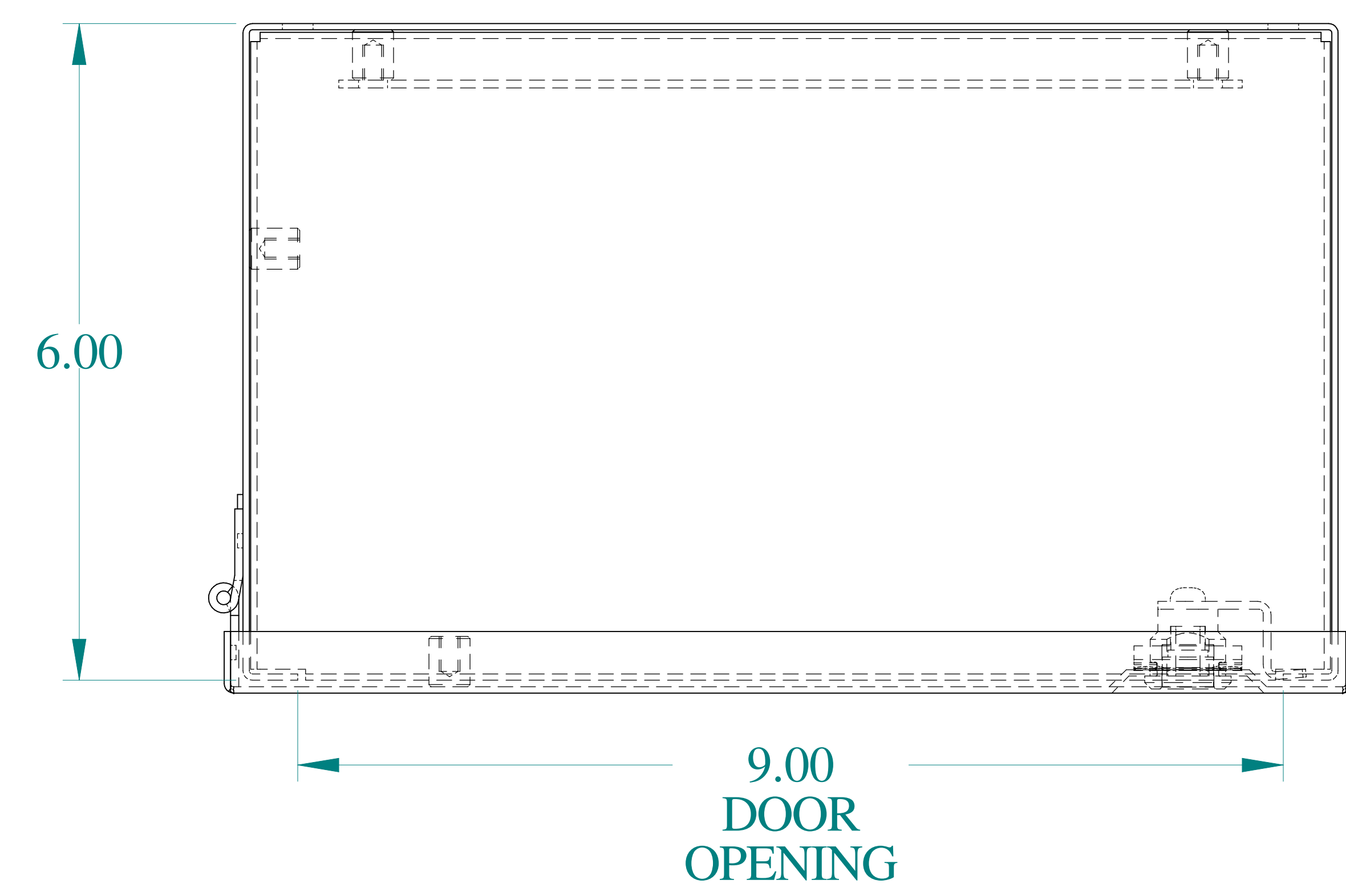
TOP VIEW
