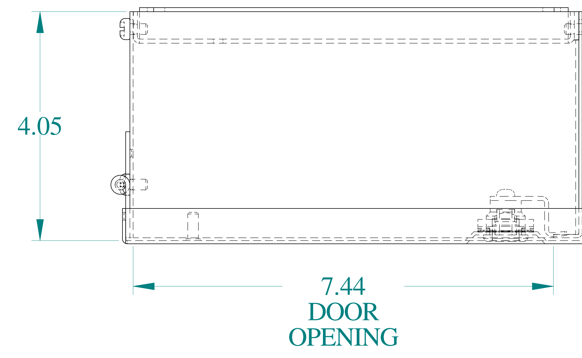
TOP VIEW
