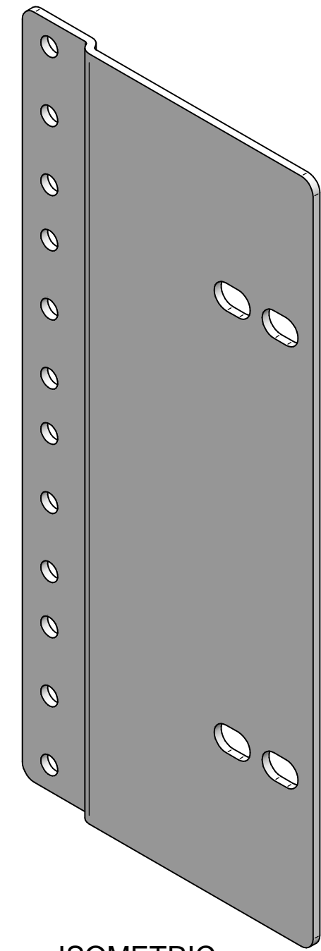
ISOMETRIC
