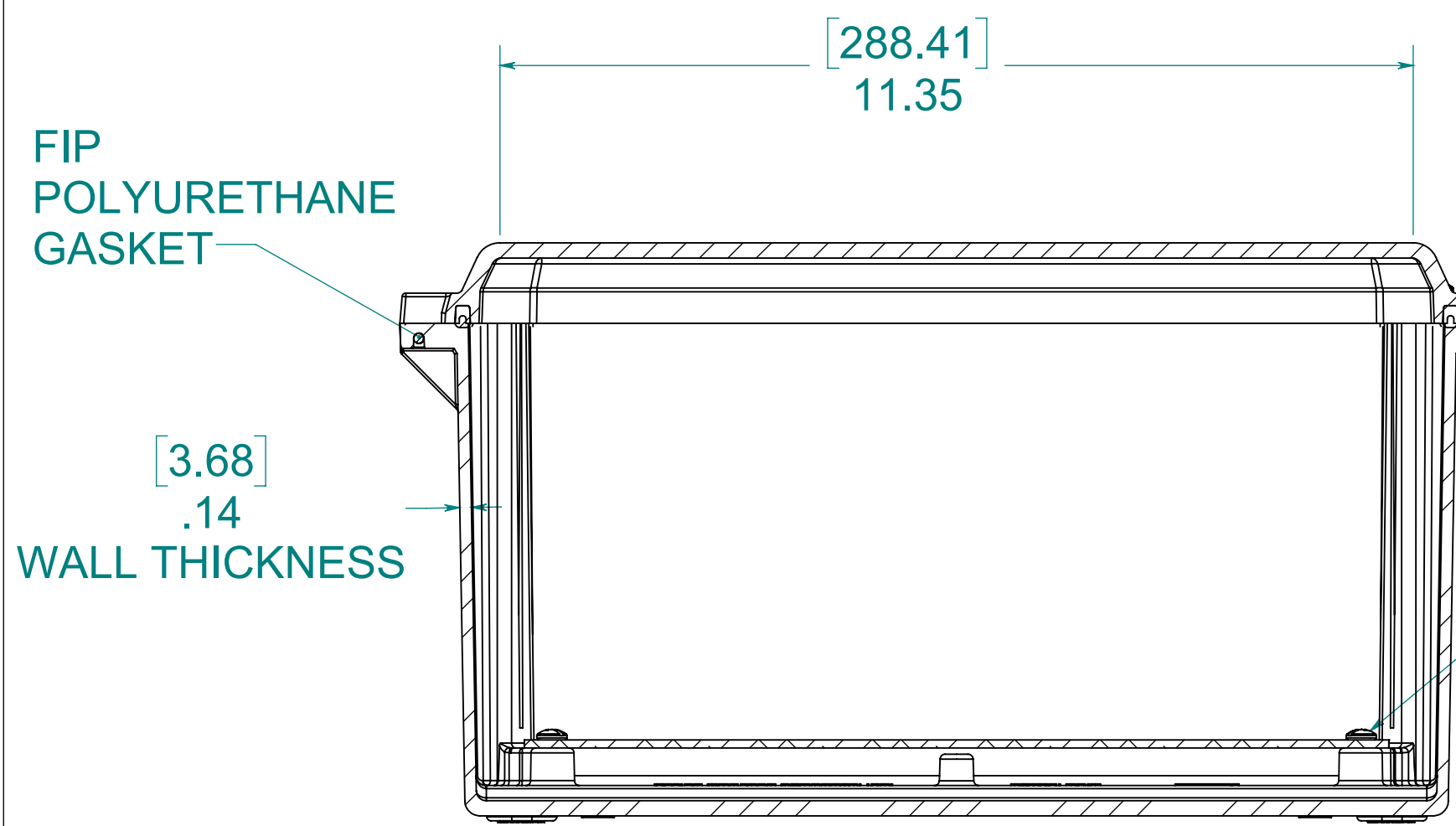
SECTION B-B
