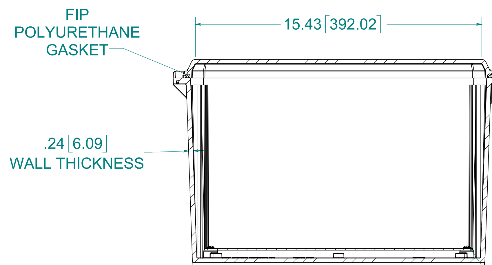
SECTION B-B
