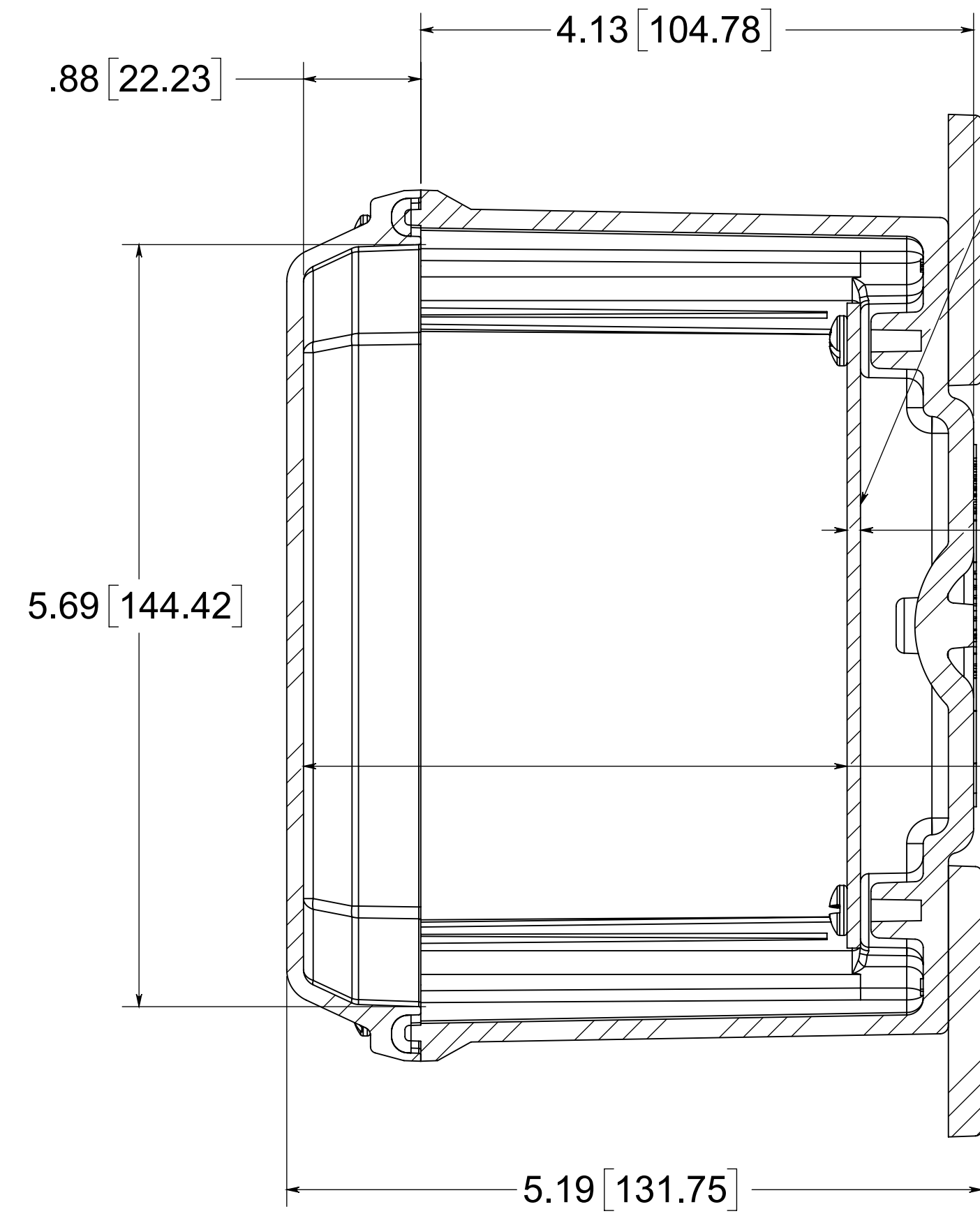
SECTION B-B
