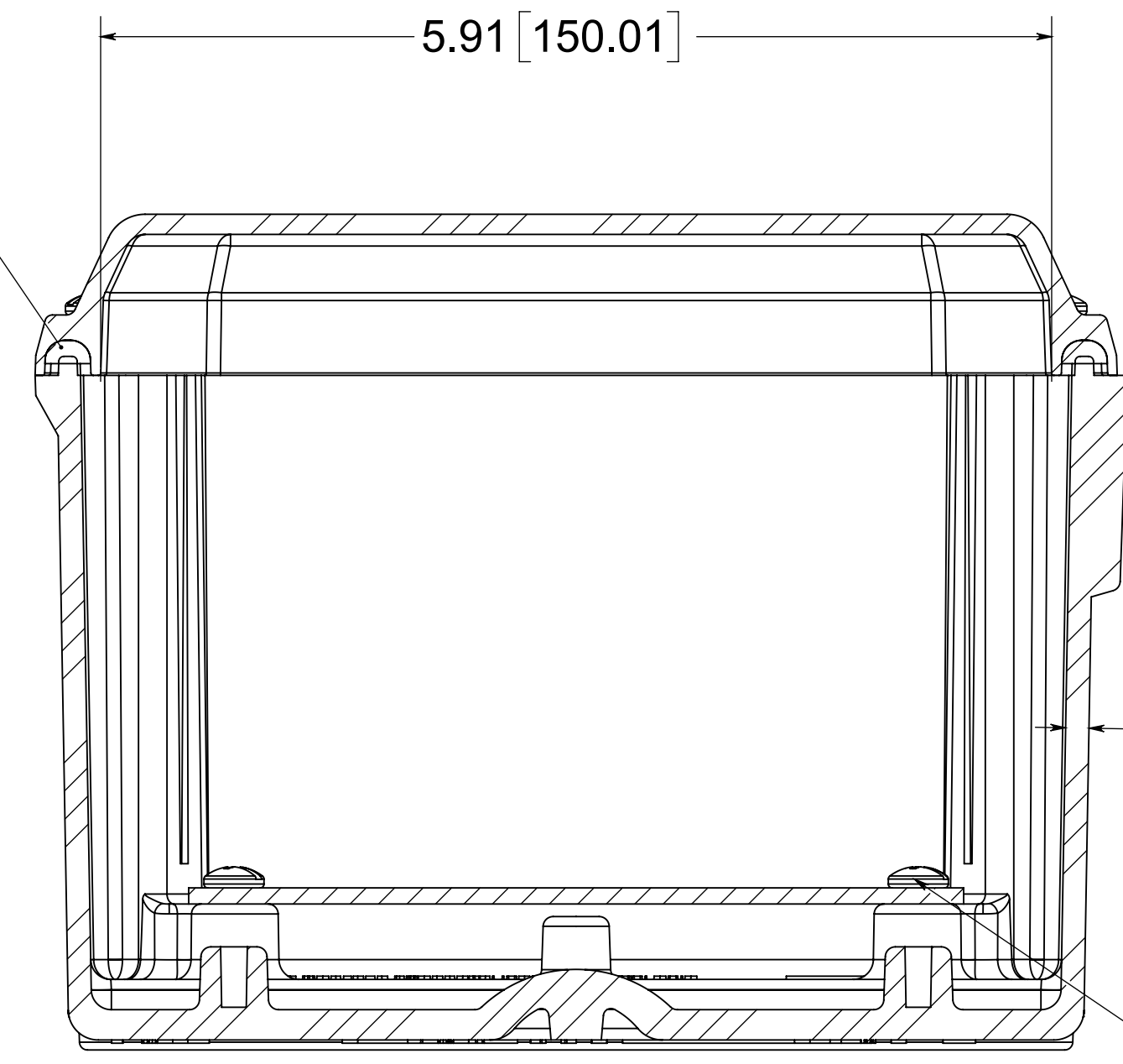
SECTION F-F
