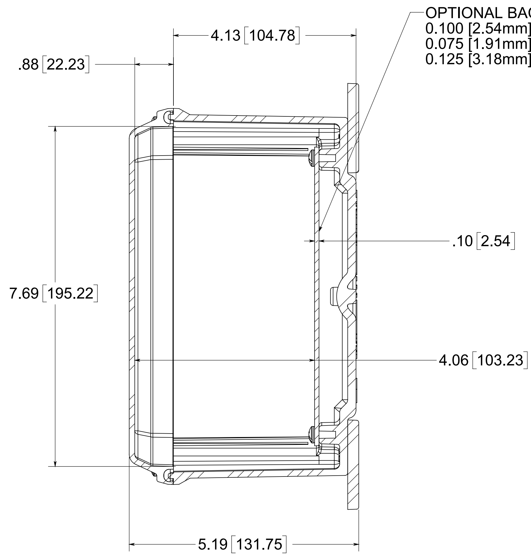
SECTION B-B
