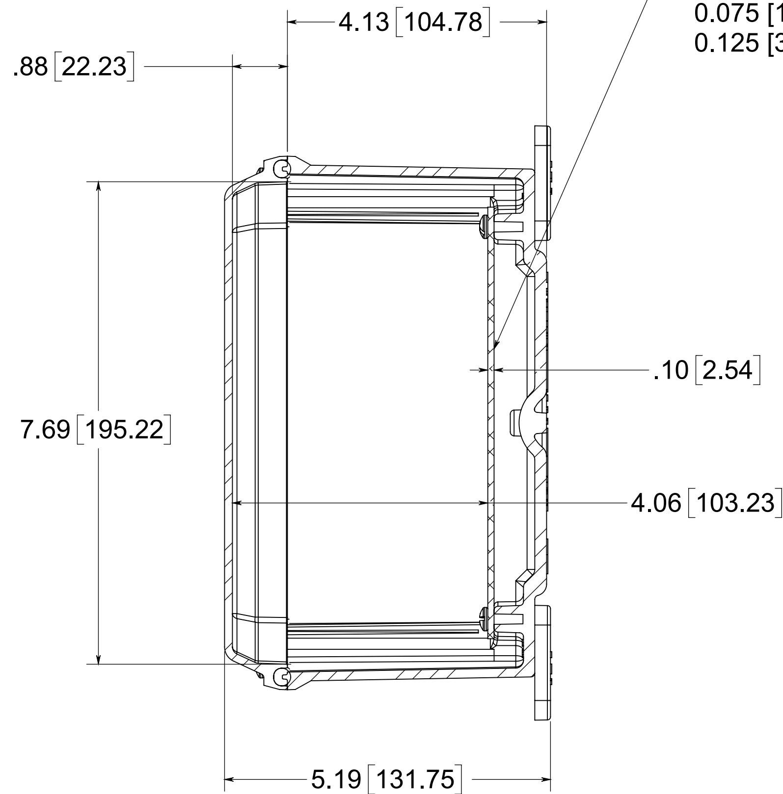
SECTION B-B
