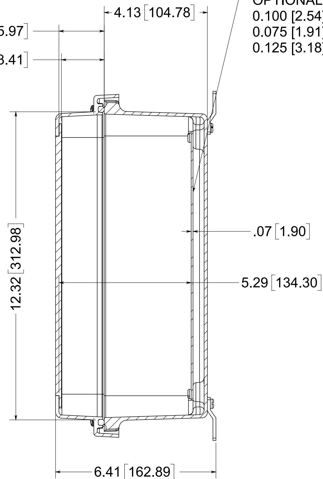
SECTION B-B
