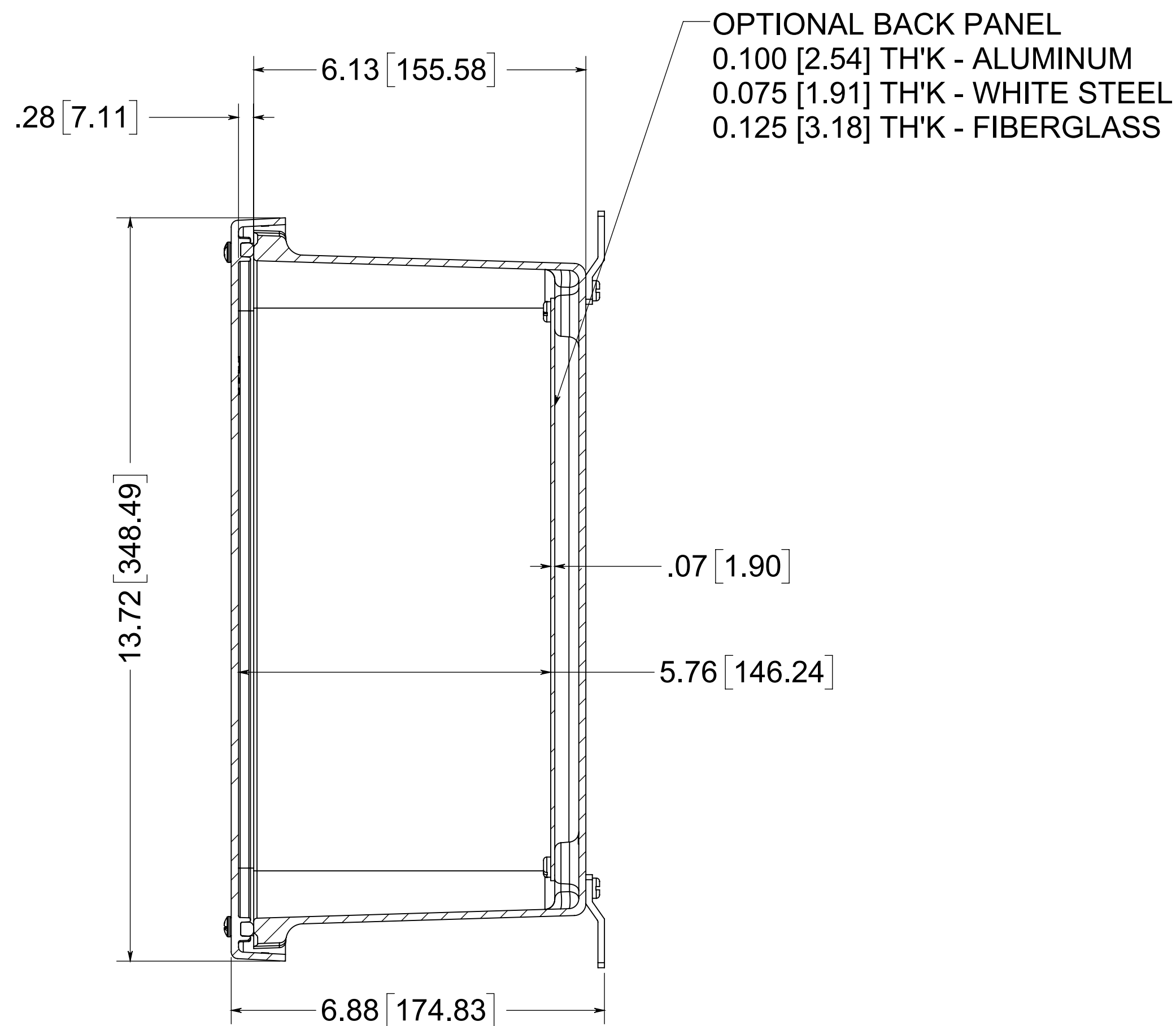
SECTION B-B
