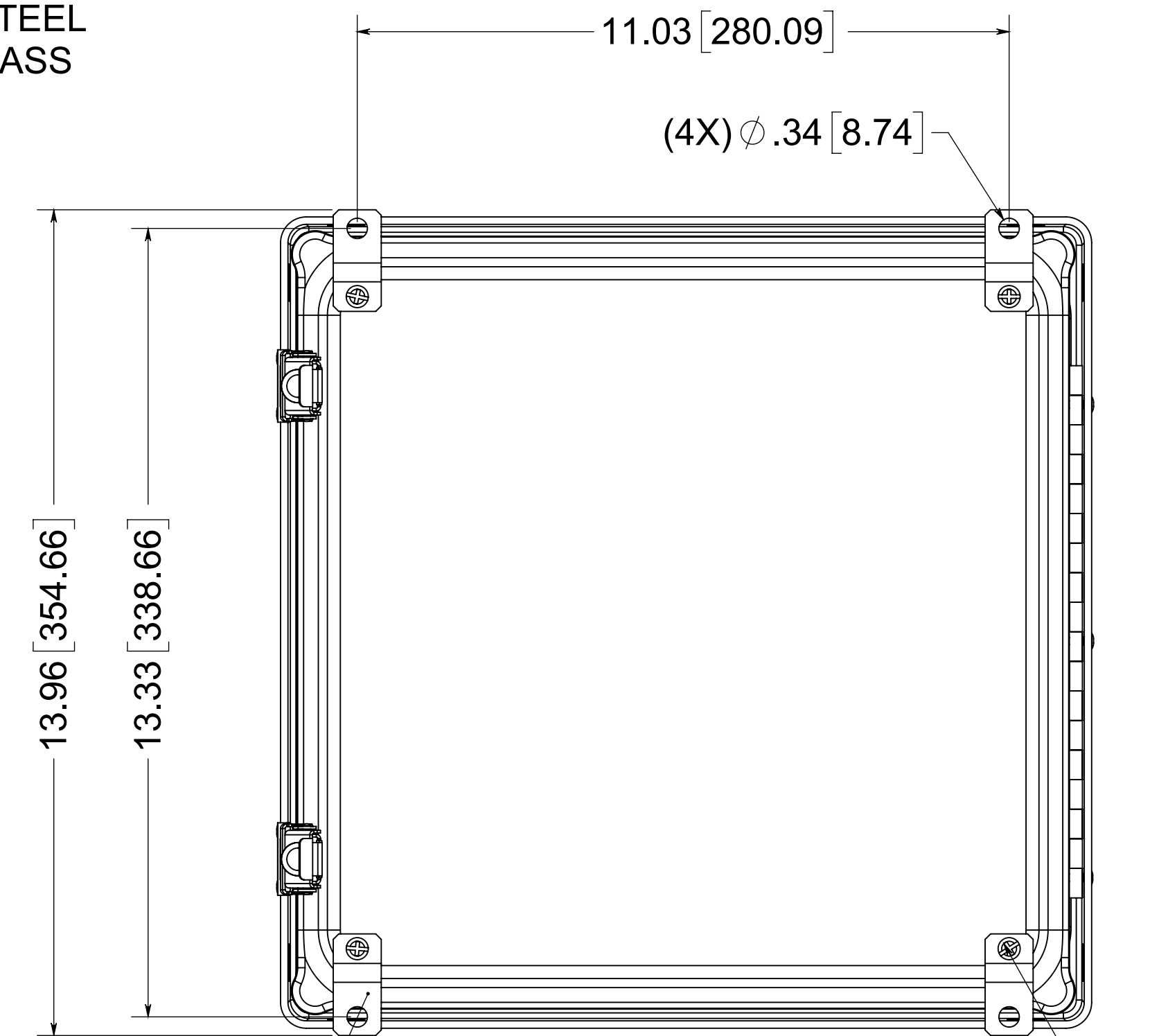
(4X) 316 STAINLESS STEEL FEET
