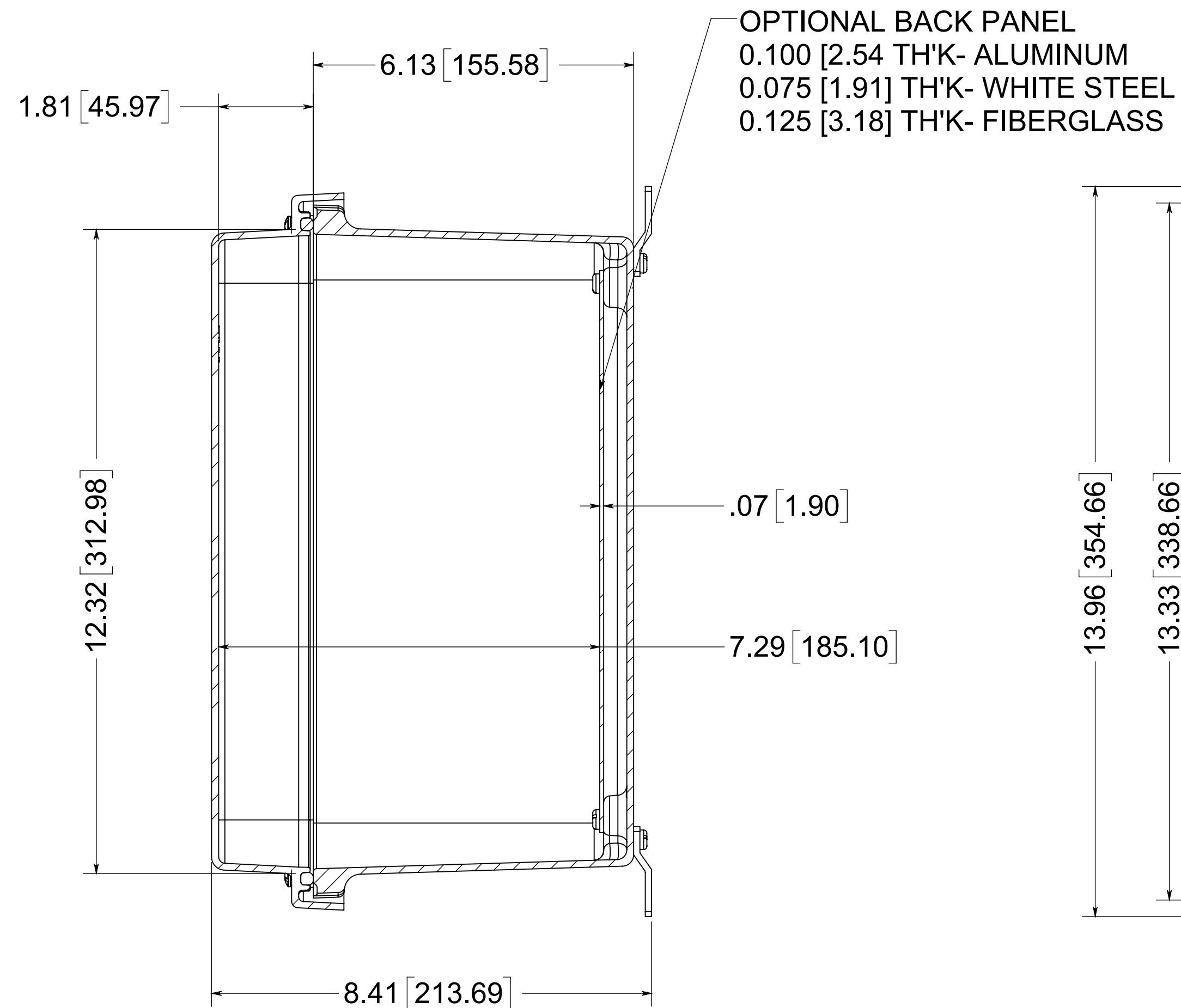
SECTION B-B
