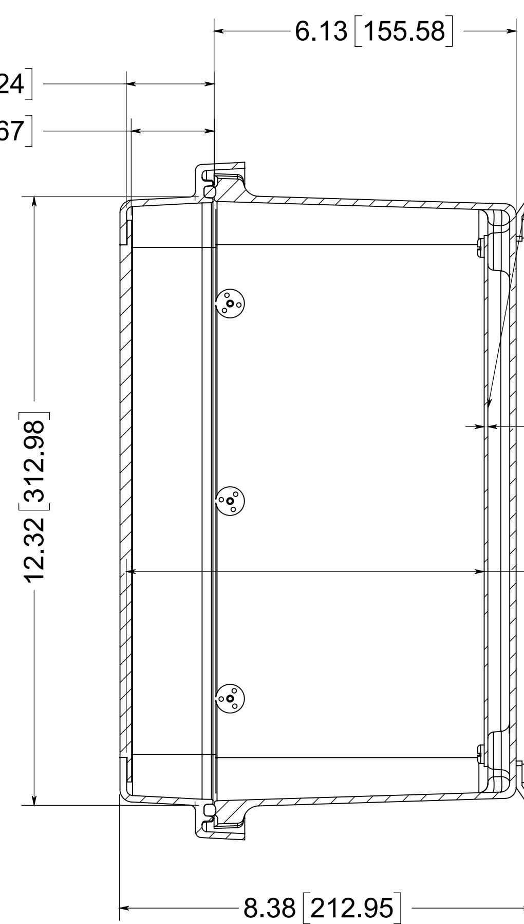
SECTION B-B
