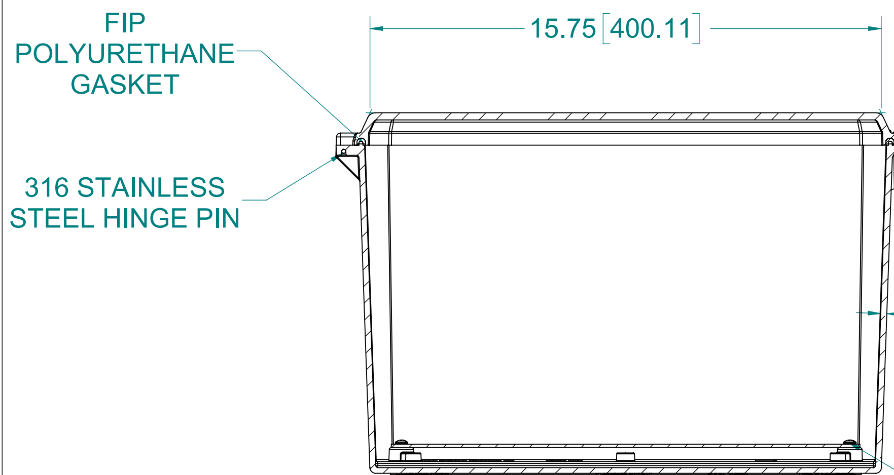
SECTION B-B
