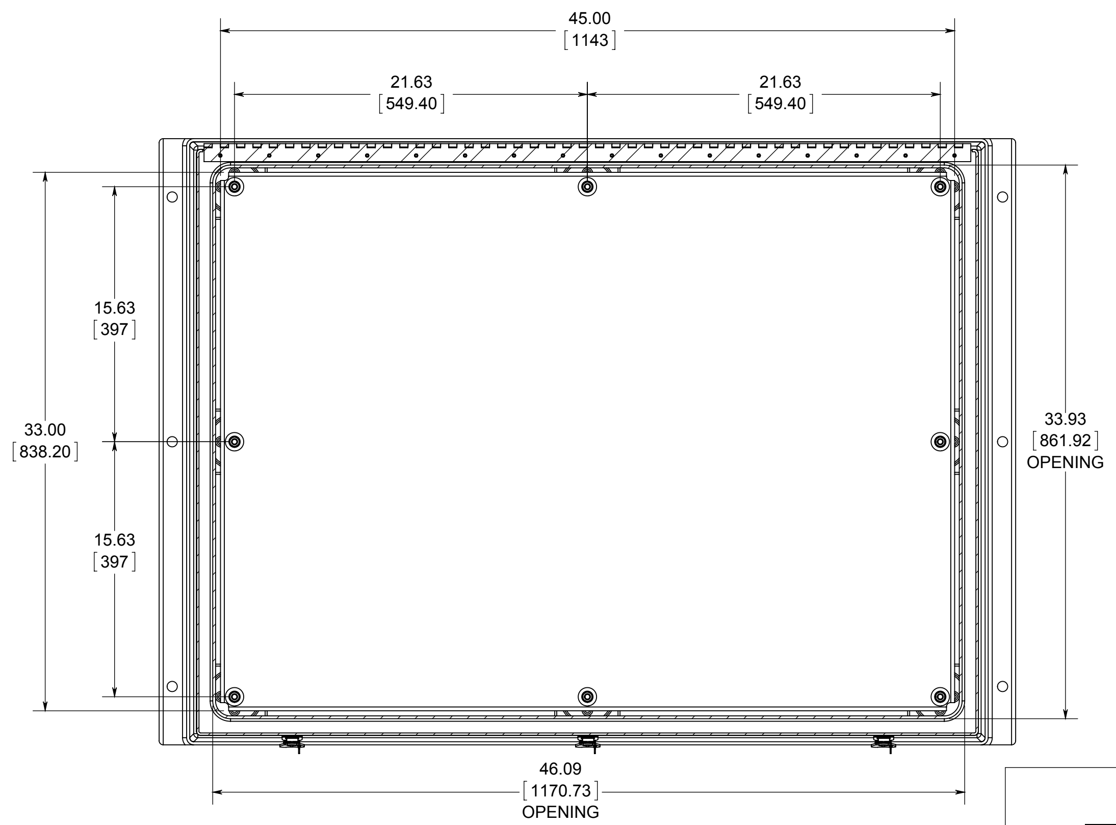
SECTION C-C TOP VIEW WITH LID AND GASKET REMOVED
