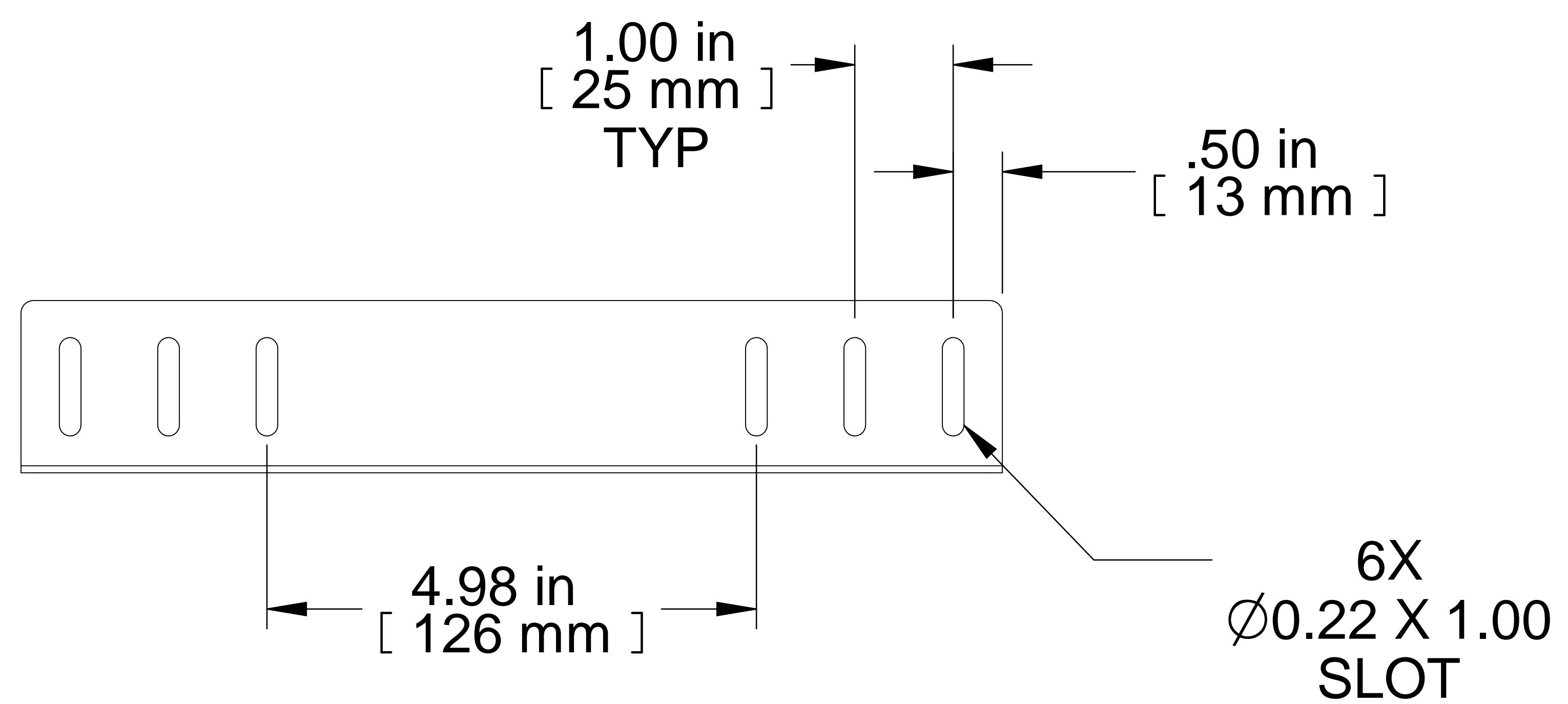
TOP VIEW
