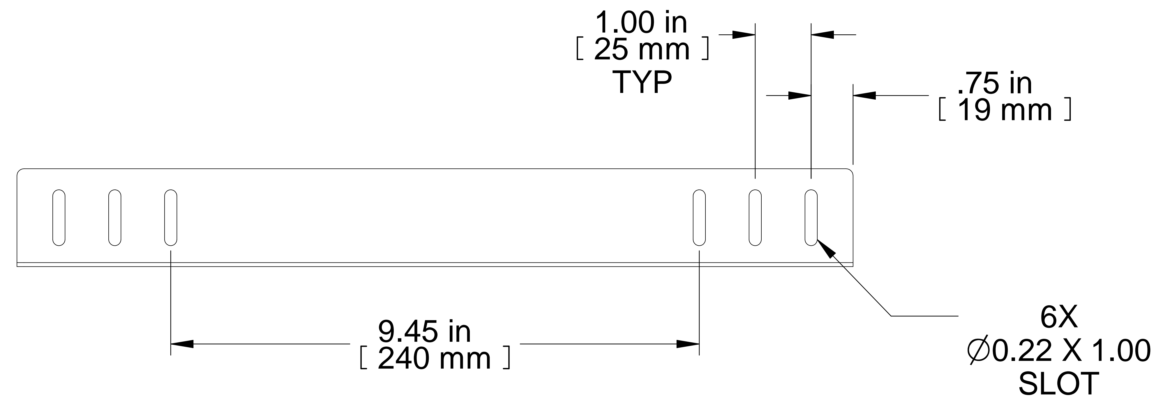
TOP VIEW
