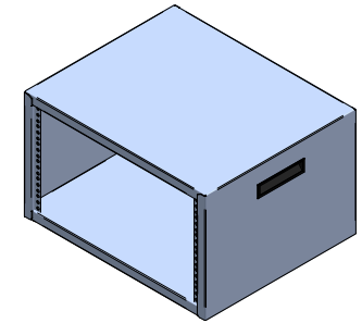
ISOMETRIC
