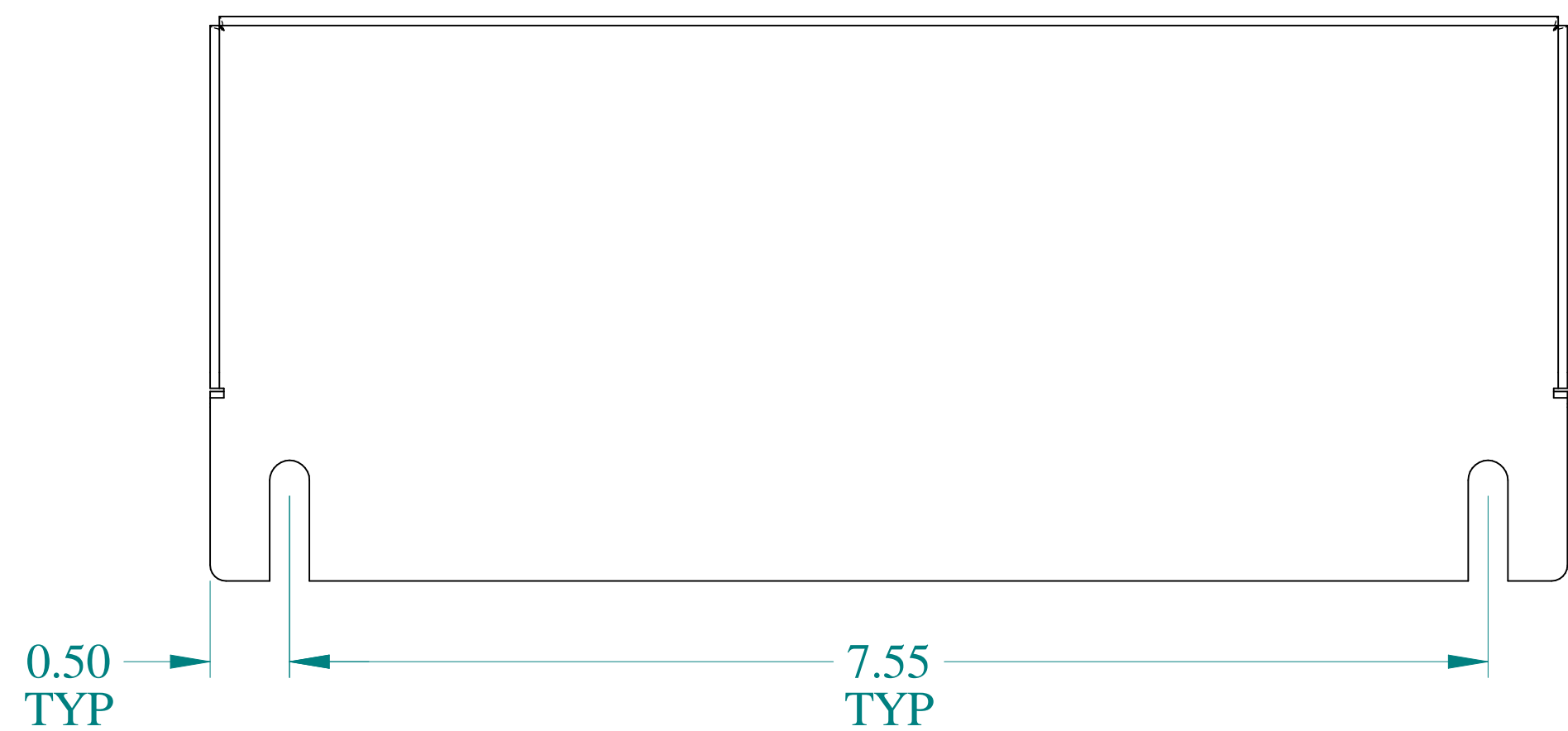
FRONT VIEW
