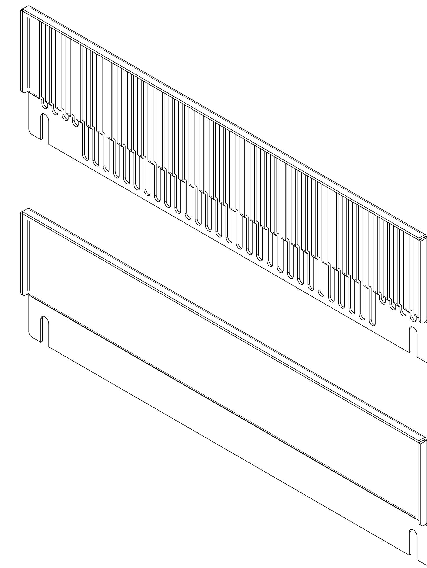
ISOMETRIC VIEW
