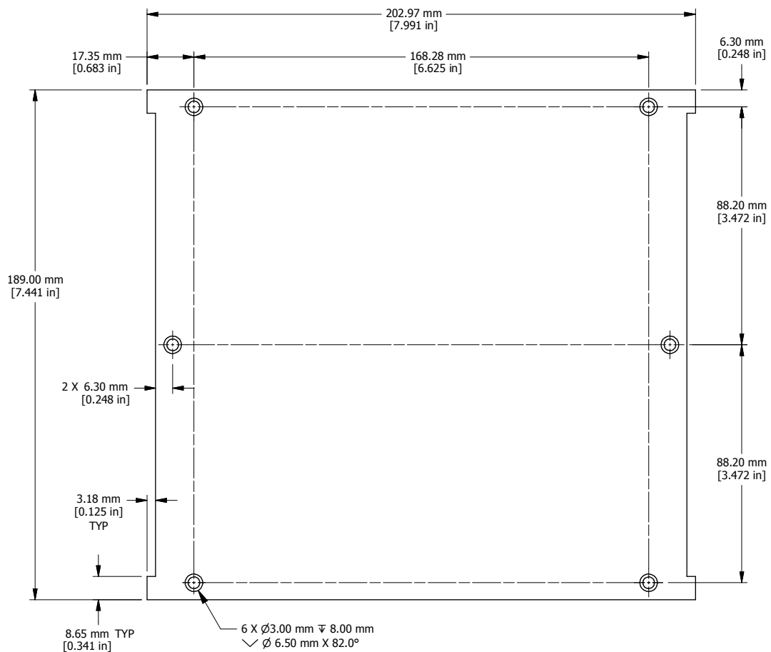
TOP VIEW
