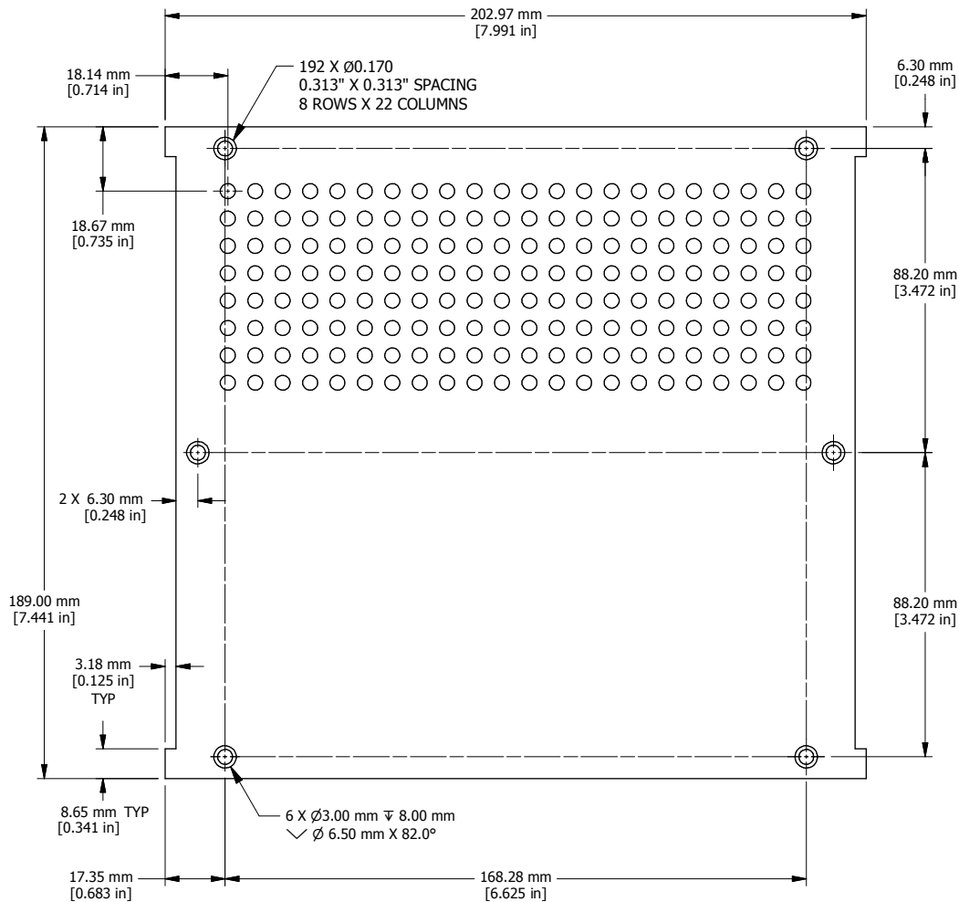
TOP VIEW
