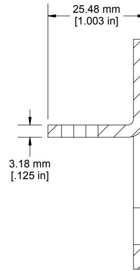
SECTION B-B
