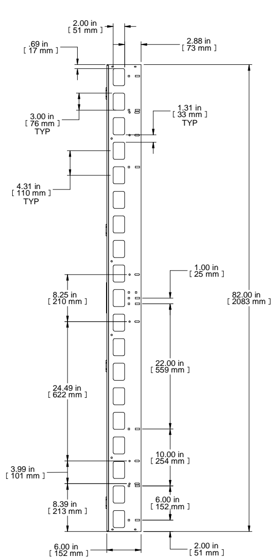
R.S. VIEW
