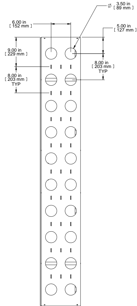
REAR VIEW
