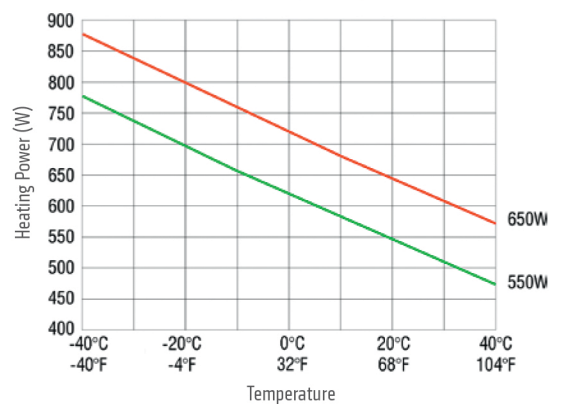
Heating Power / Ambient Temperature (@ 60 Hz)
