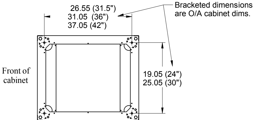
BOTTOM VIEW OF C4 CABINET
