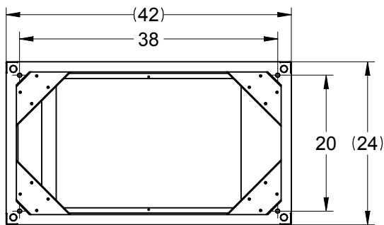
BOTTOM VIEW OF DC100 CABINET
