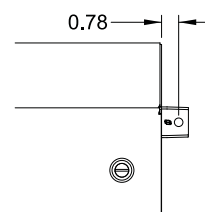
Mounting Foot Detail
