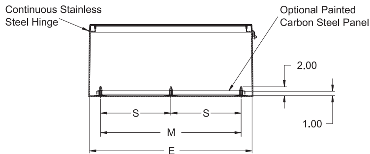
End View
